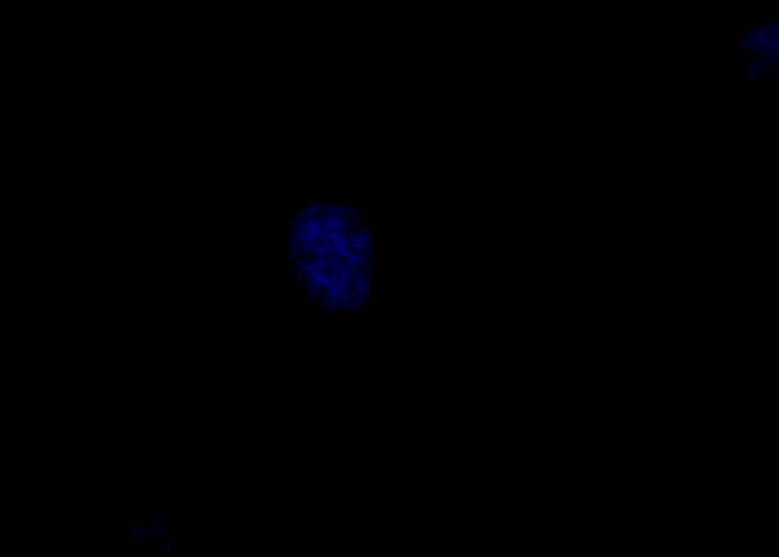
Figure 3(B2) - DAPI
