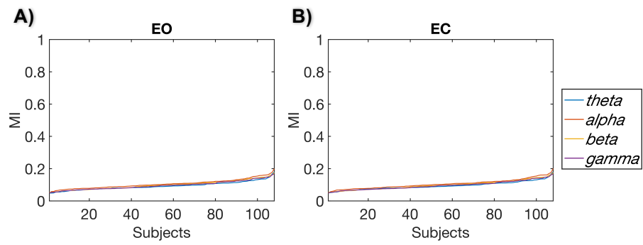
Figure S3: Mirkin index (MI) between partitions of observed networks and a consensus partition of the synthetic networks for k = 3 . We selected \tau = 1 as a resolution parameter to construct the consensus partition. Similar results were obtained for \tau > 1 (data not shown here)
