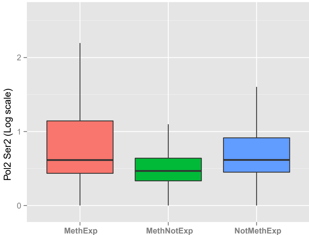
Supplemental Figure 10. The evidence of transcriptional elongation based on PolII-Ser2 signals (Y-axis) in the segment region associated with three gene groups, MethExp (pink), MethNotExp (green) and NotMethExp (blue) (X-axis).
