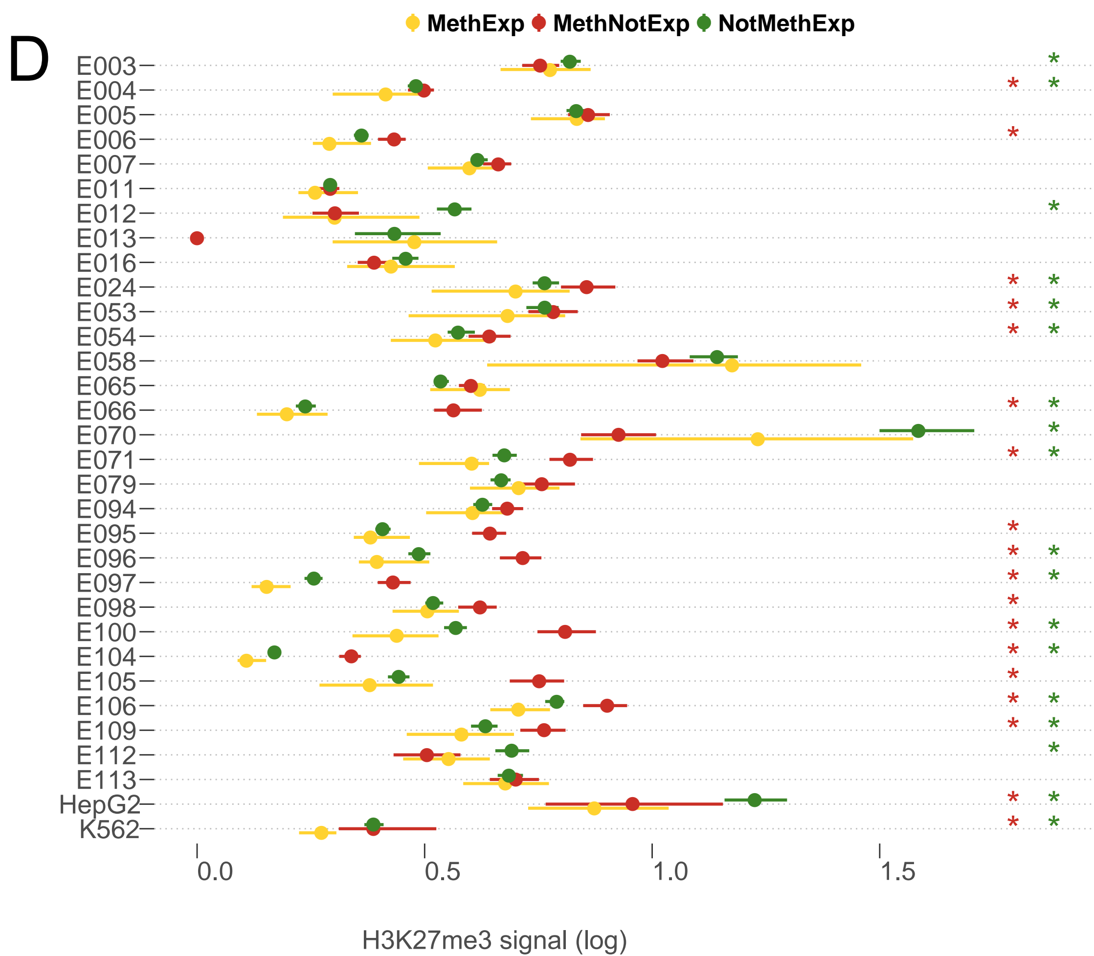
Supplemental Figure 8. Active and repressive marks at the distal CGIs. (A) Median DNase signal, (B) median H3K4me3 signal, (C) median H3K9ac signal, (D) median H3K27me3 signal, (E) median H3K9me3 signal, and 95% CI (X-axes) at the distal CGIs associated with MethExp (yellow), MethNotExp (red) and NotMethExp (green) genes across several tissue types (Y-axes).
