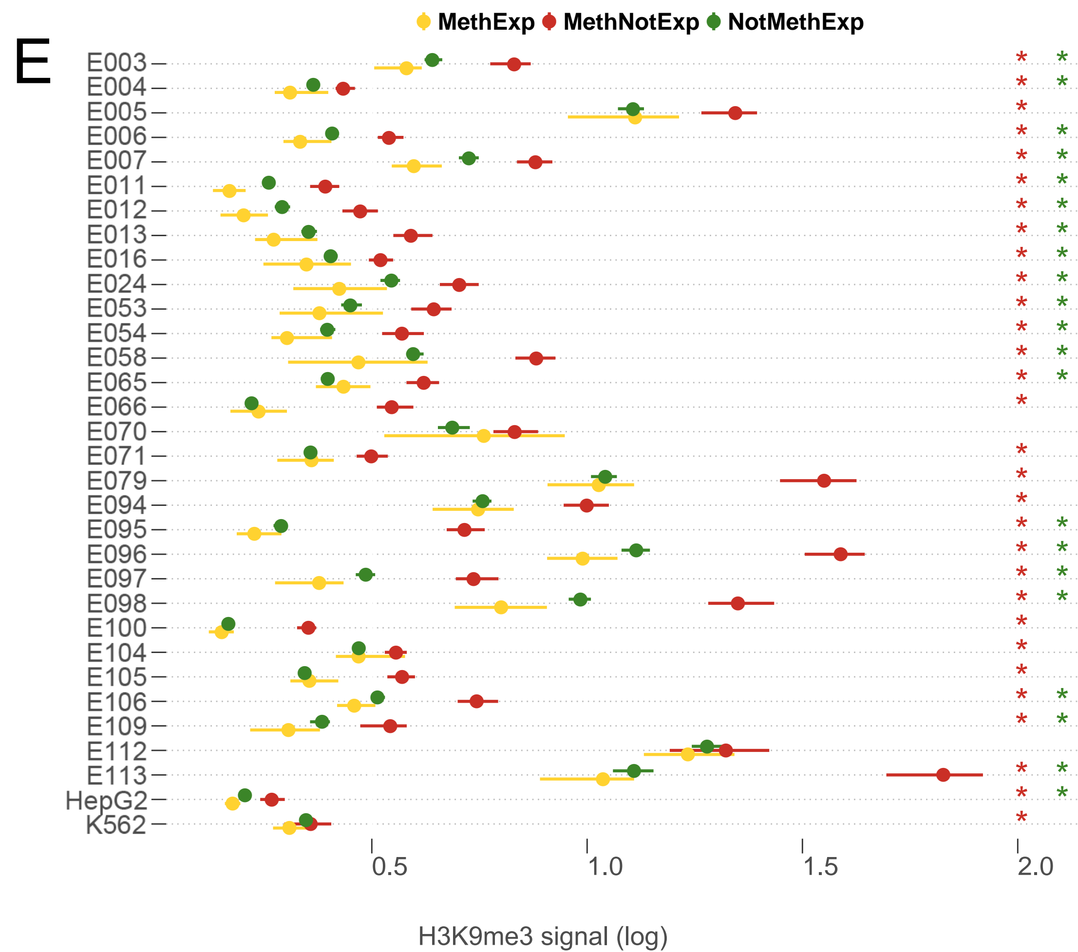
Supplemental Figure 8. Active and repressive marks at the distal CGIs. (A) Median DNase signal, (B) median H3K4me3 signal, (C) median H3K9ac signal, (D) median H3K27me3 signal, (E) median H3K9me3 signal, and 95% CI (X-axes) at the distal CGIs associated with MethExp (yellow), MethNotExp (red) and NotMethExp (green) genes across several tissue types (Y-axes).
