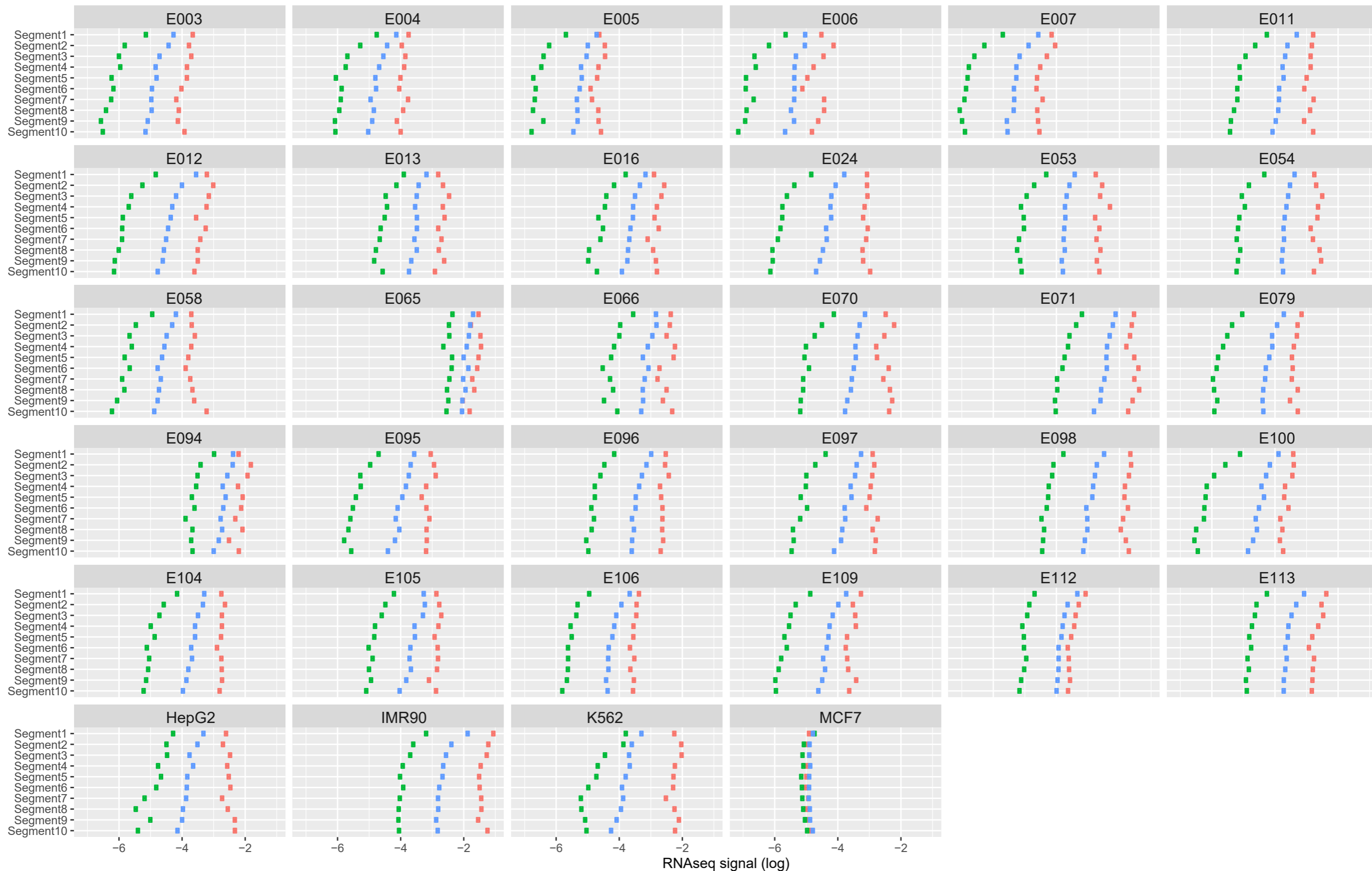
Supplemental Figure 9a. Median RNA-seq signal (RPKM) (X-axes; log transformed) in each of 10 equal bins of the segment region associated with MethExp (pink), MethNotExp (green) and NotMethExp (blue) genes across 34 tissue types.
