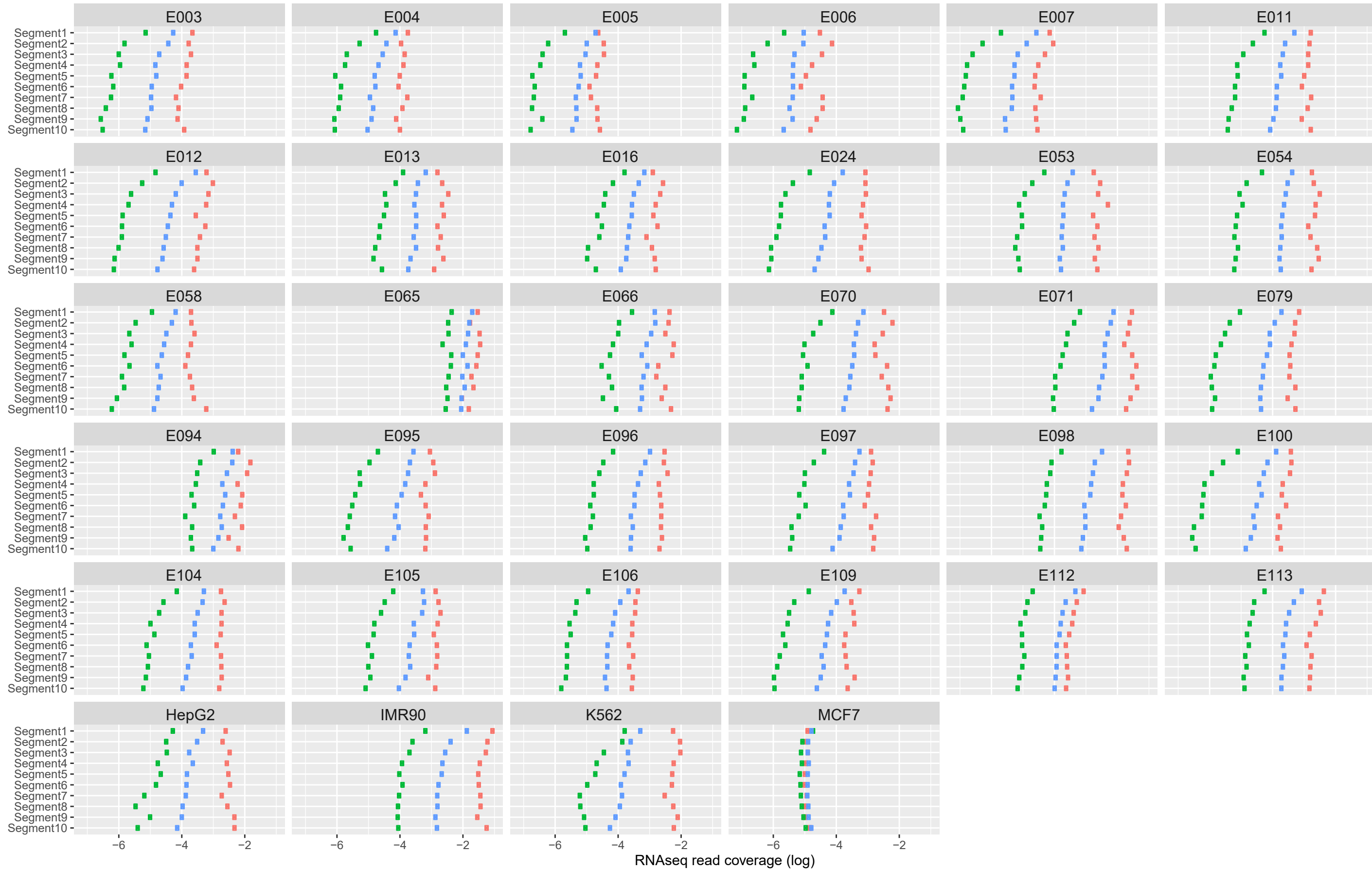
Supplemental Figure 9b. Median RNA-seq read coverage (X-axes; log transformed) in each of 10 equal bins of the segment region associated with MethExp (pink), MethNotExp (green) and NotMethExp (blue) genes across 34 tissue types.
