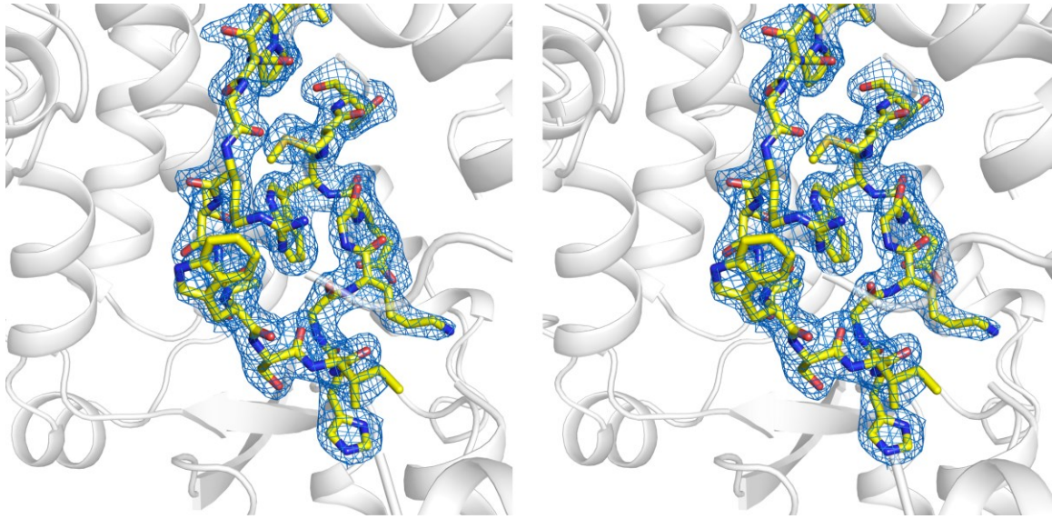
Supplementary Figure 1: Stereo view of the priming loop electron density map ( 2F_o - F_c ) of ZIKV NS5 RdRp, with 1.0 sigma.
