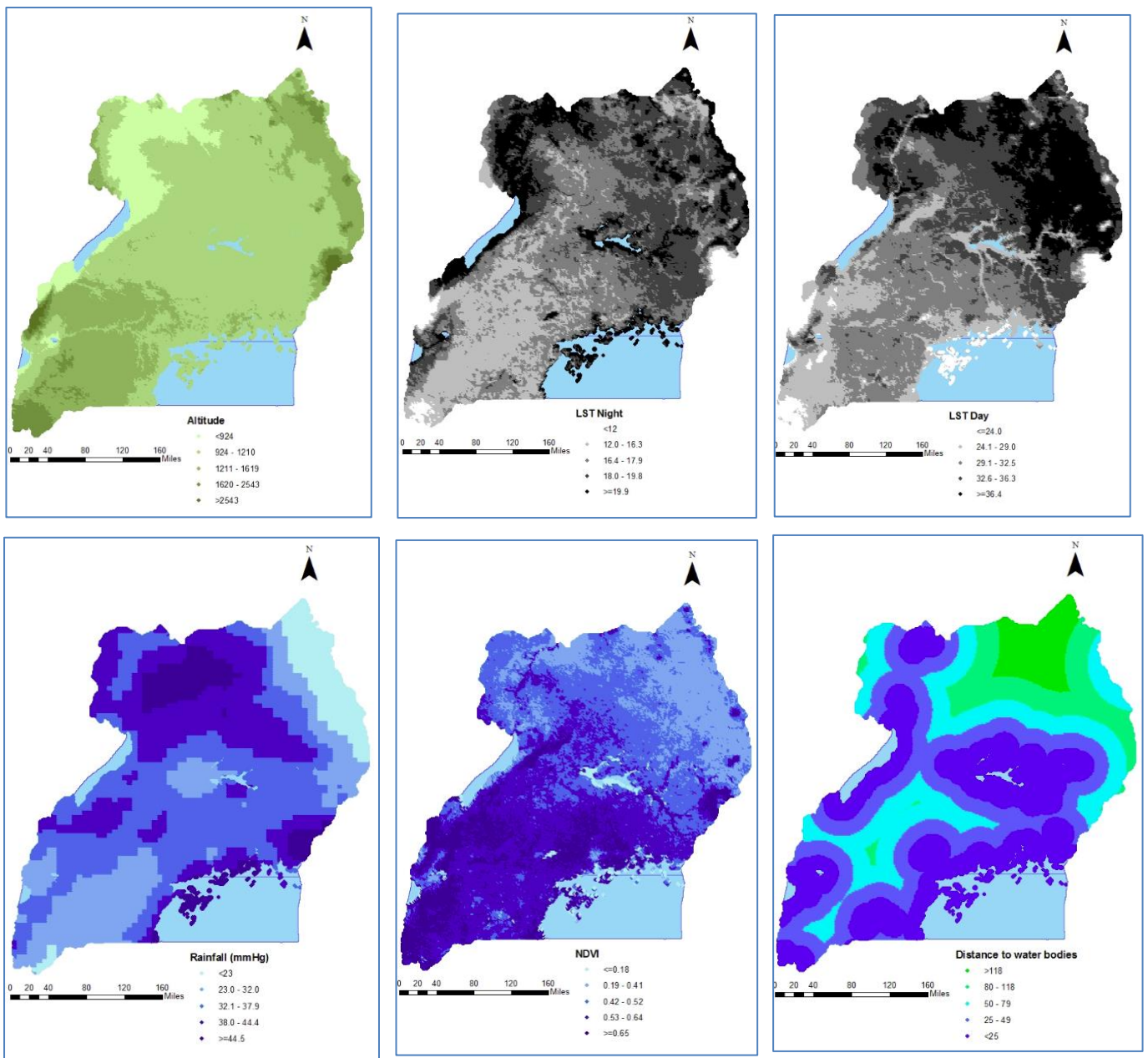
S2Fig: Distribution of climatic/environmental factors in Uganda in 2014
