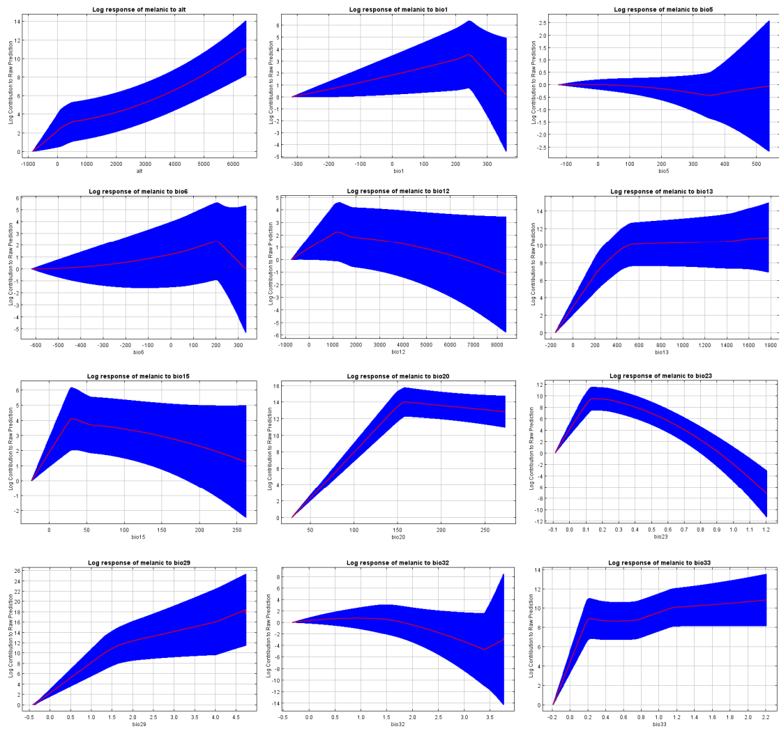
S3 Fig - Response curves observed in the Maxent analysis for each environmental predictor used to construct the melanistic model.
