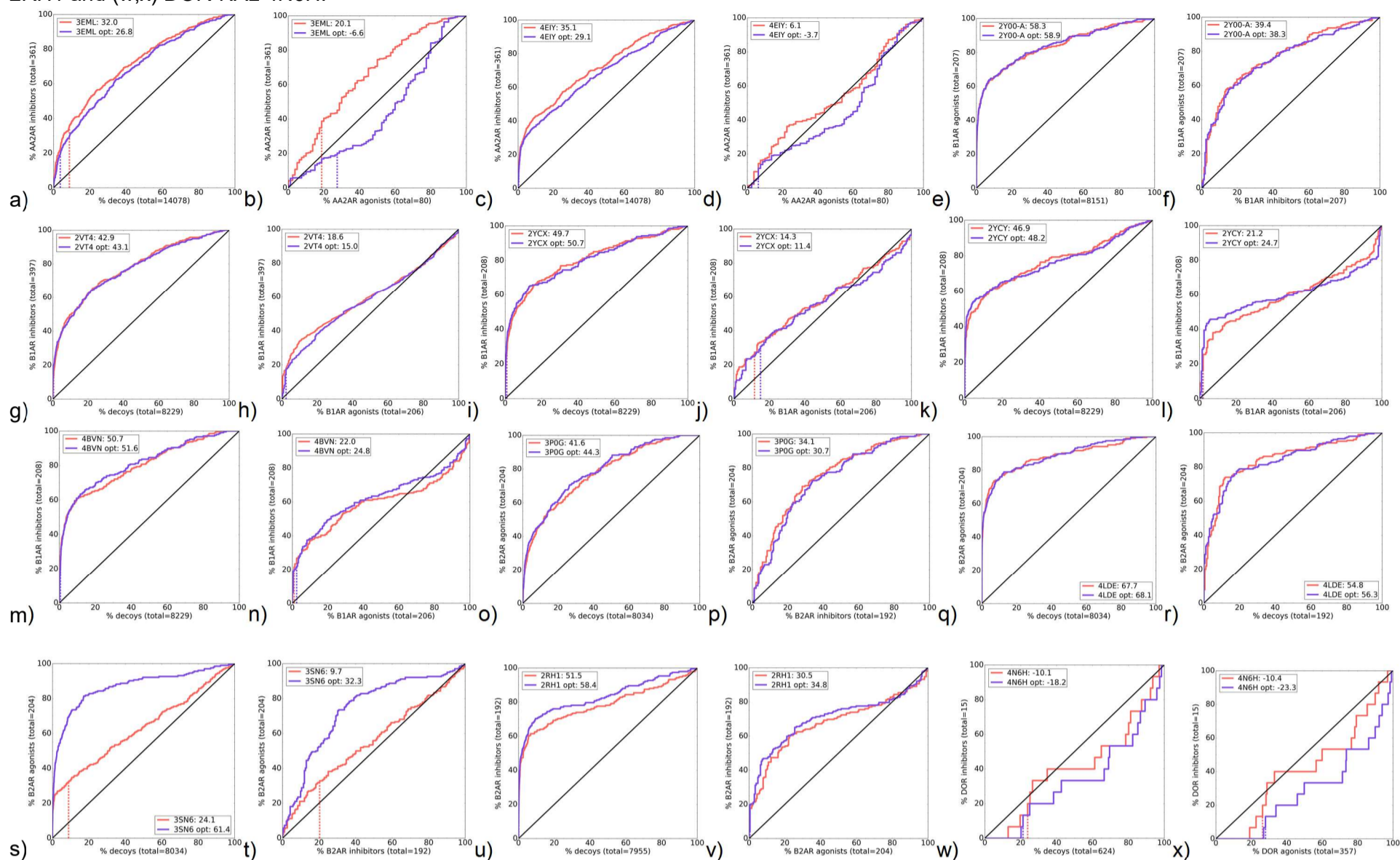
S1 Fig. Comparison of VS performance with and without hydrogen bond optimization. The known ligands vs. decoys and agonist vs. inhibitors (or vice versa) are compared respectively for (a,b) AA2AR-ZM 3EML, (c,d) AA2AR-ZM 4E1Y, (e,f) B1AR-DOB 2Y00-A, (g,h) B1AR-CYP 2VT4, (i,j) B1AR-CYP 2YCX, (k,l) B1AR-CYP 2YCY, (m,n) B1AR-CYP 4BVN, (o,p) B2AR-BI 3P0G, (q,r) B2AR-BI 4LDE, (s,t) B2AR-BI 3SN6, (u,v) B2AR-CAR 2RH1 and (w,x) DOR-NAL 4N6H.
