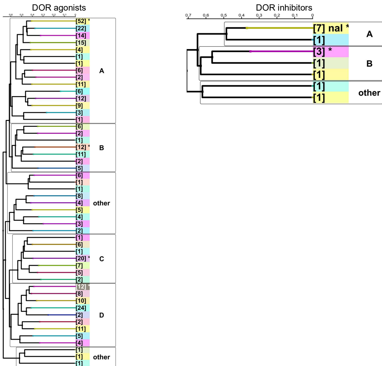
S6 Fig. Dendrogram of the ligand chemotypes for DOR. The number of ligands within each branch is noted. Clusters used in VS are circled and named, and the co-crystal X-ray ligand's position is identified. The asterisk denotes the location of the chemotype cluster center for its respective chemotype cluster, no cluster center is provided for the cluster 'other'.
