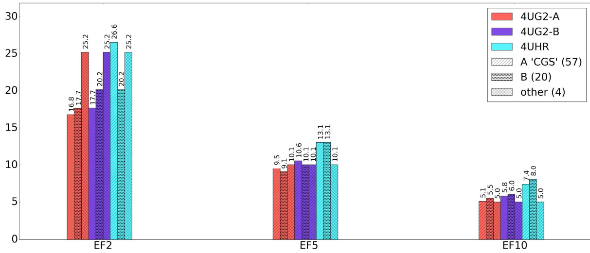
S7 Fig. Enrichment factors of AA2AR known agonist chemotypes for CGS-bound AA2AR binding pockets (4UG2-A, 4UG2-B, 4UHR). Enrichment factors at EF2, EF5 and EF10 using the 2D racemic ligand library.
