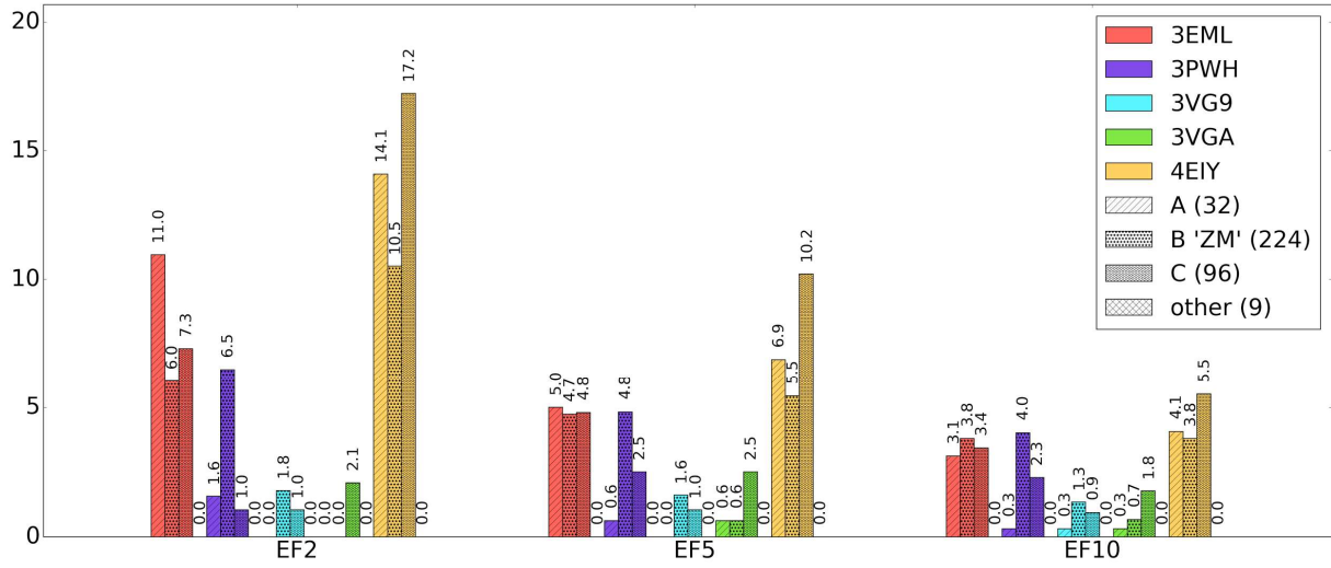
S9 Fig. Enrichment factors of AA2AR known inhibitor chemotypes for ZM-bound AA2AR binding pockets (3EML, 3PWH, 3VG9, 3VGA, 4EIY). Enrichment factors at EF2, EF5 and EF10.
