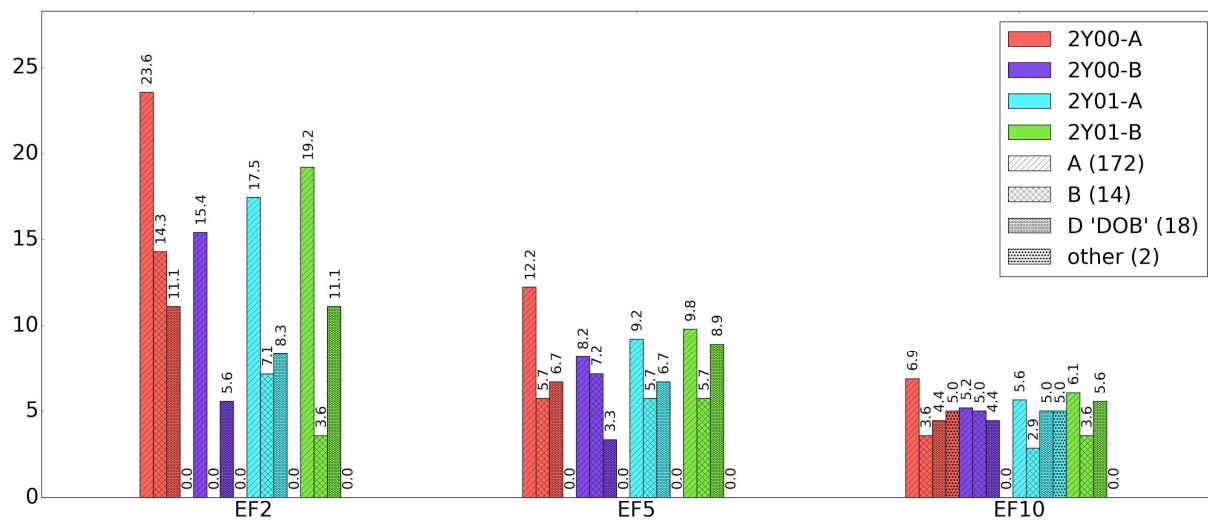
S10 Fig. Enrichment factors of B1AR known agonist chemotypes for DOB-bound B1AR binding pockets (2Y00-A, 2Y00-B, 2Y01-A, 2Y01-B). Enrichment factors at EF2, EF5 and EF10.
