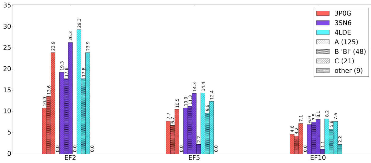
S12 Fig. Enrichment factors of B2AR known agonist chemotypes for BI-bound B2AR binding pockets (3P0G, 3SN6, 4LDE). Enrichment factors at EF2, EF5 and EF10.
