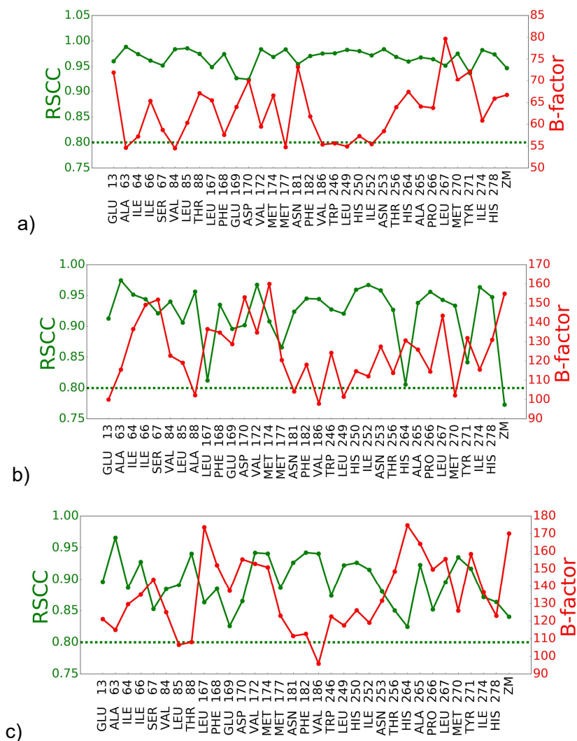
S15 Fig. RSCC and B-factor plots for AA2AR ZM-bound binding pockets. Assessment of local model quality for: a) 3EML, b) 3PWH, c) 3VG9, d) 3VGA and e) 4EIY. Real-space correlation coefficient (green) and B-factor values (red) are shown for all residues of the binding pocket and the bound ligand ZM. A green dotted line cutoff value of 0.8 highlights low RSCC values.
