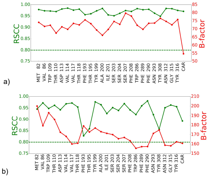
S19 Fig. RSCC and B-factor plots for B2AR CAR-bound binding pockets. Assessment of local model quality for: a) 2RH1 and b) 4GBR. Real-space correlation coefficient (green) and B-factor values (red) are shown for all residues of the binding pocket and the bound ligand CAR. A green dotted line cutoff value of 0.8 highlights low RSCC values.
