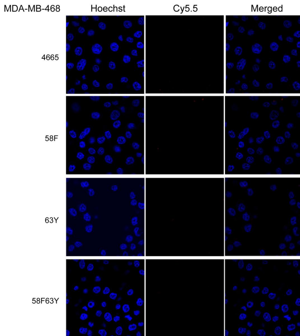
S3 Fig. Confocal fluorescence imaging analysis of the MDA-MB-468 cell line with low HER2 expression after incubating with peptides labeled with Cy5.5.
