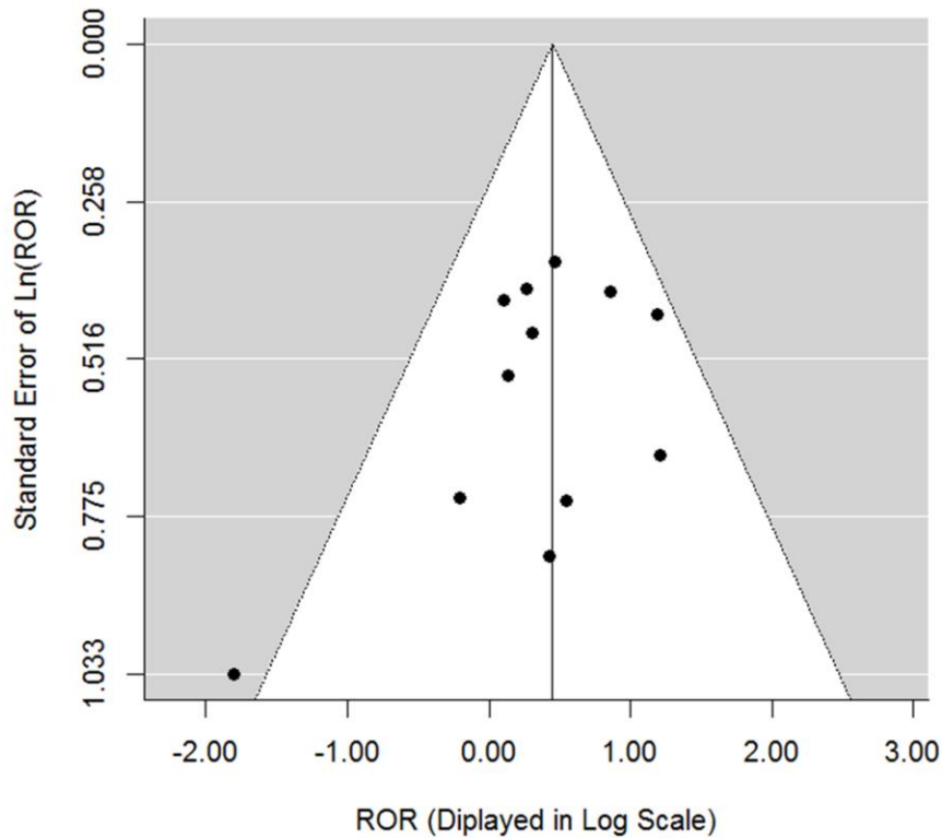
Supplementary Figure 1. Funnel plot for detecting reporting bias of hyponatremia adverse events.
