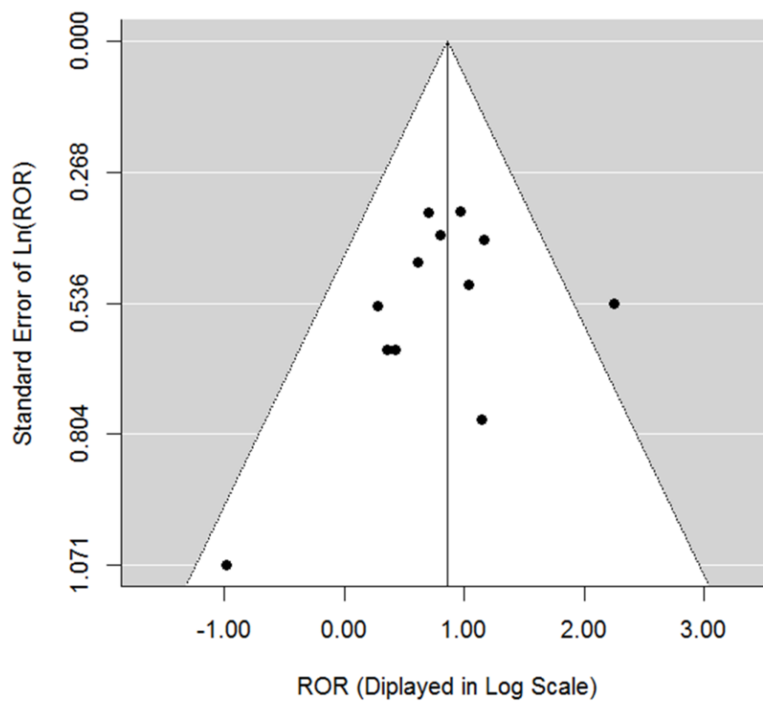
Supplementary Figure 2. Funnel plot for detecting reporting bias of hypokalemia adverse events.
