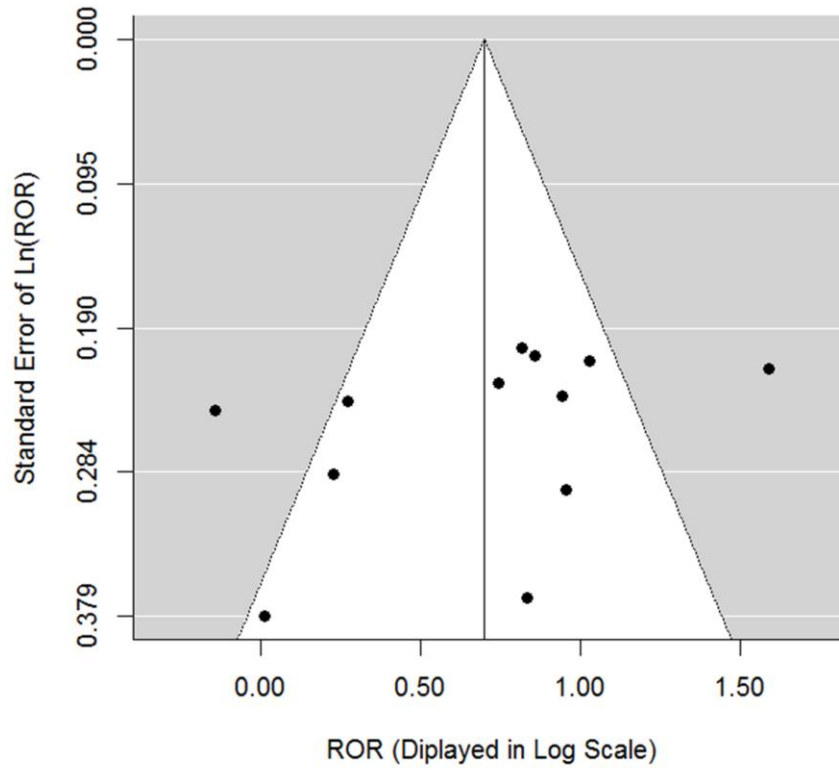
Supplementary Figure 3. Funnel plot for detecting reporting bias of dehydration adverse events.
