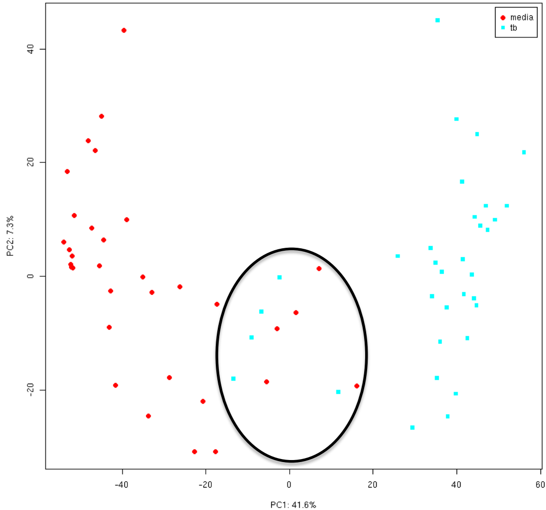
S1 Figure. PCA Reveals Batch Effect. Principal components analysis of the full dataset of 13 TSTNEG and 20 TSTPOS subjects revealed ten outlier samples that are poorly resolved by PC1 (black circle). These ten samples are pairs (media or M.tb treated) from five individuals (3 TSTNEG and 2 TSTPOS) that were processed on the same day. Because of the obvious batch effect, these samples were removed and not included in the final dataset.
