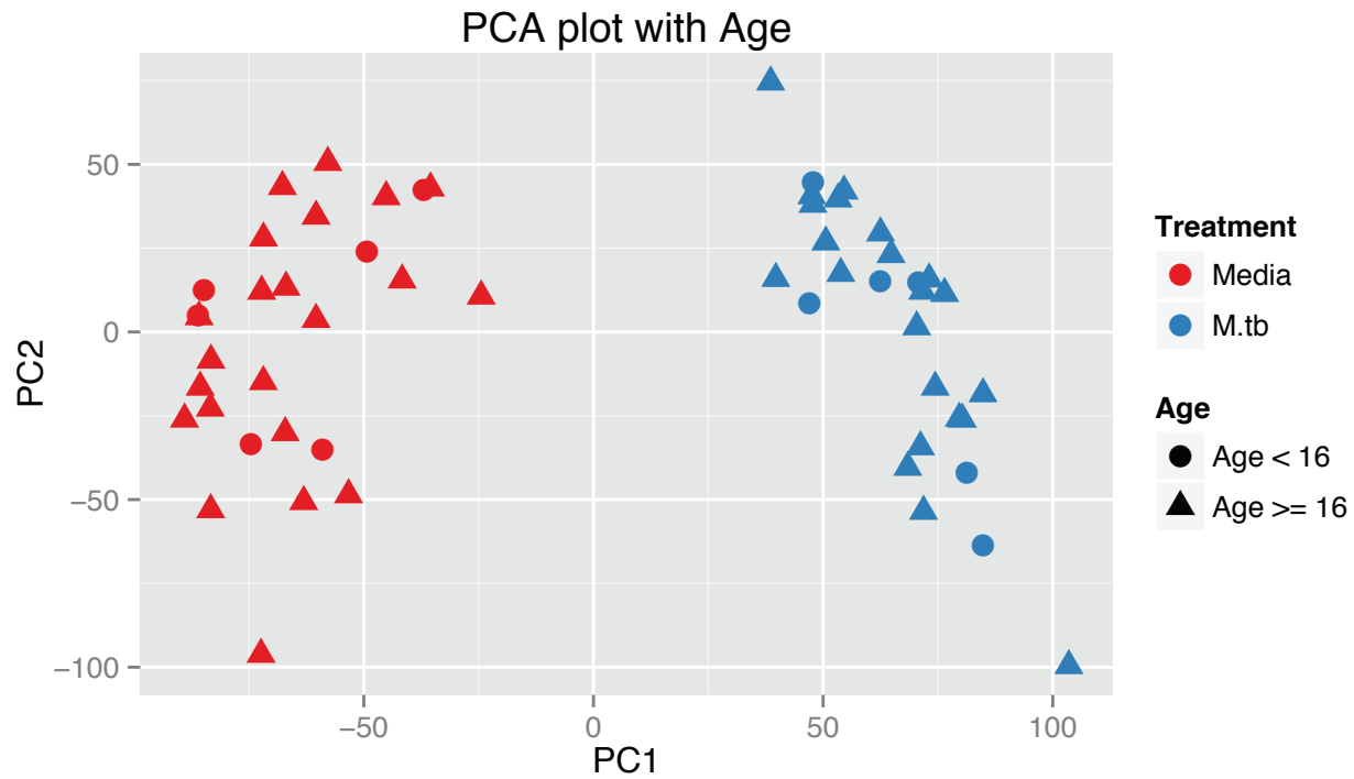
Supplementary Figure 3. Principal Components Plot stratified by Age and Treatment. The data shown in Figure 1B of the main text was re-labelled using age instead of TST status. Samples arising from 6 study subjects under the age of 16 are evenly distributed among those greater than 16 years of age
