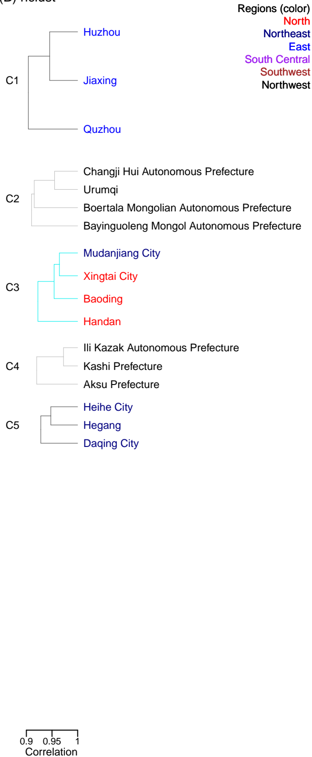
(B) hclust
