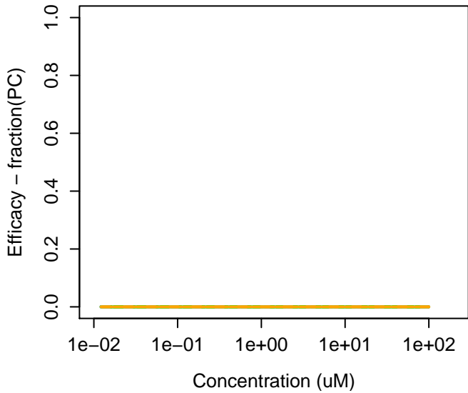
6088-51-3 : 6-Hydroxy-2-naphthyl disulfide
