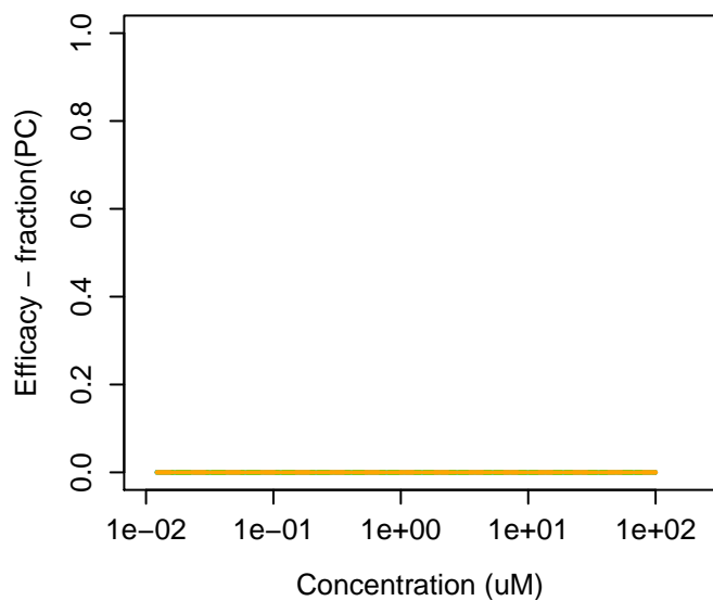
78-82-0 : 2-Methylpropanenitrile
