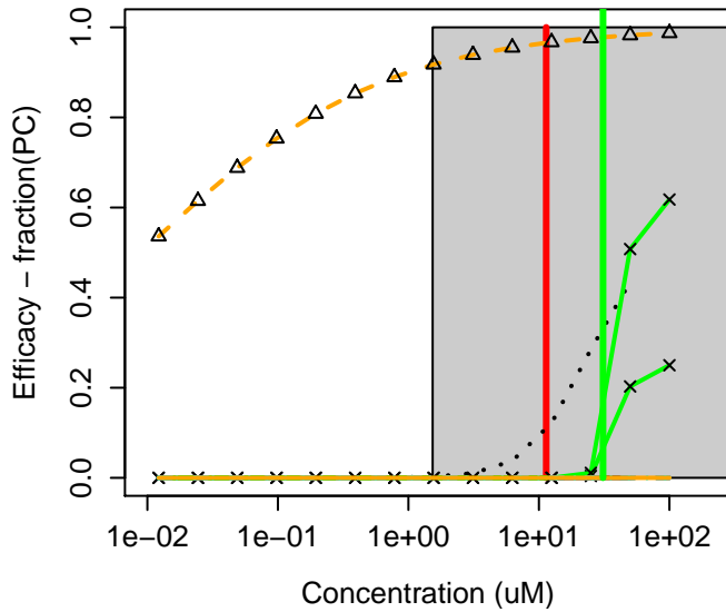
104-54-1 : 3-Phenyl-2-propen-1-ol
