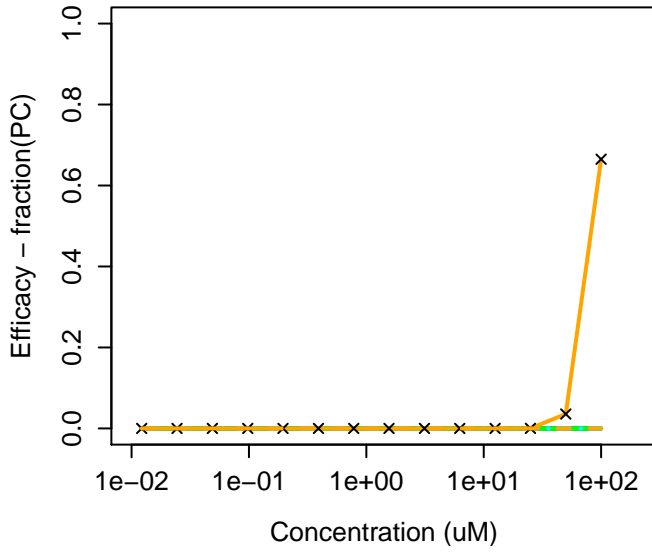
156-60-5 : (E)-1,2-Dichloroethylene
