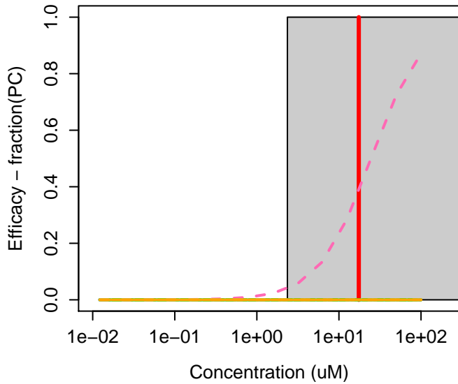
6789-88-4 : Hexyl benzoate
