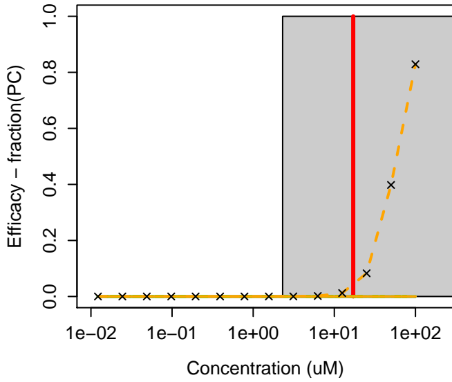
58-18-4 : 17-Methyltestosterone
