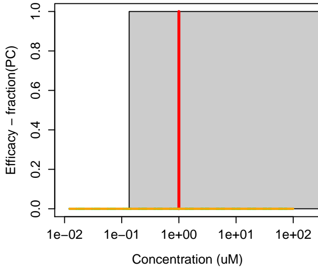
112-00-5 : Dodecyltrimethylammonium chloride
