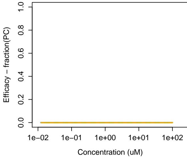
110-42-9 : Methyl decanoate
