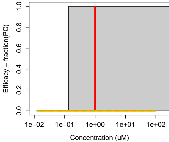
7173-51-5 : Didecyldimethylammonium chloride
