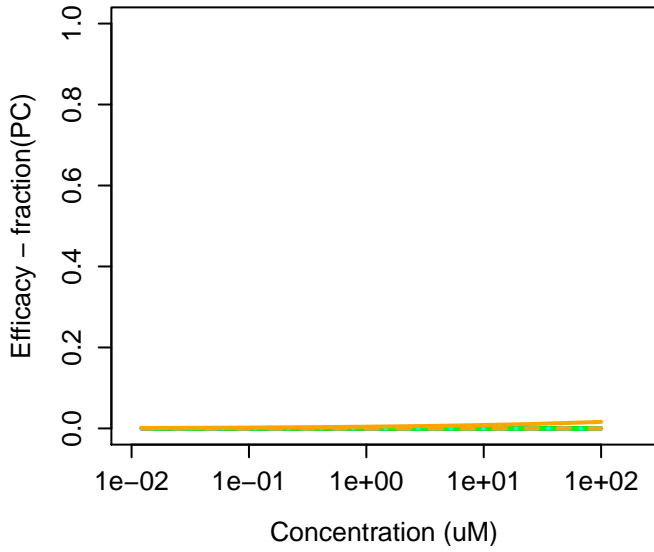
51632-16-7 : 1-(Bromomethyl)-3-phenoxybenze
