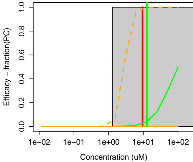
534-13-4 : N,N'-Dimethylthiourea
