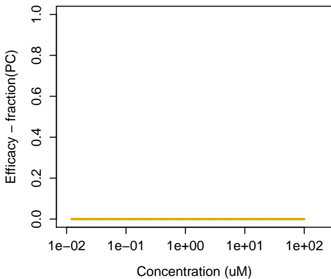
527680-56-4 : PHA-00568487
