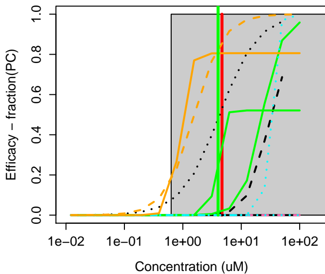
81741-28-8 : Tributyltetradecylphosphonium chlor
