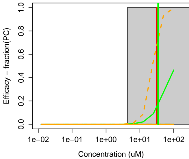
88-60-8 : 2-tert-Butyl-5-methylphenol
