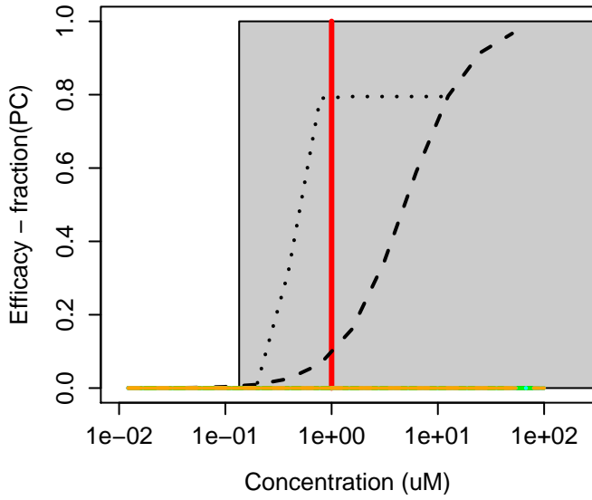
64-67-5 : Diethyl sulfate
