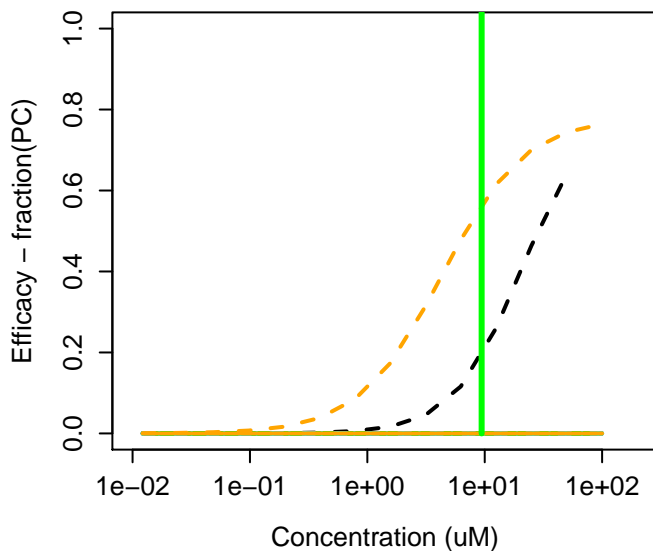
119-93-7 : 3,3'-Dimethylbenzidine
