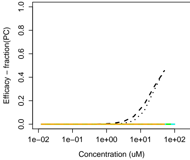
6153-64-6 : Oxytetracycline dihydrate
