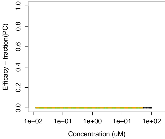
650-51-1 : Sodium trichloroacetate
