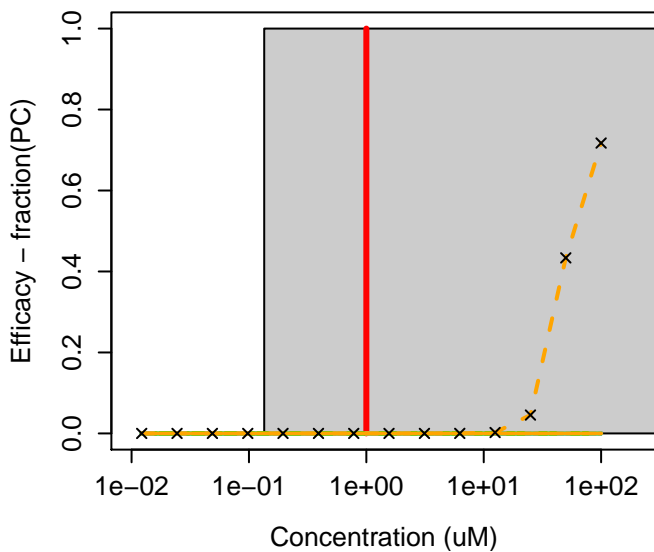
6610-29-3 : N-Methylhydrazinecarbothioamide
