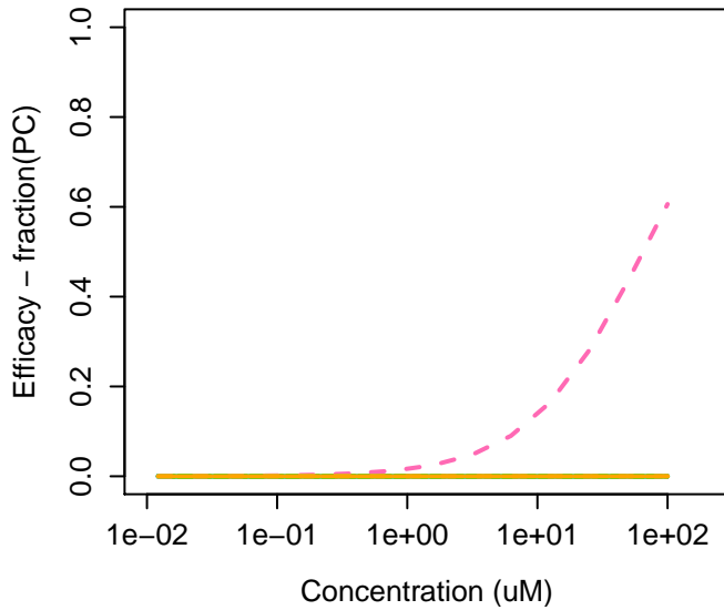
89-72-5 : 2-(Butan-2-yl)phenol
