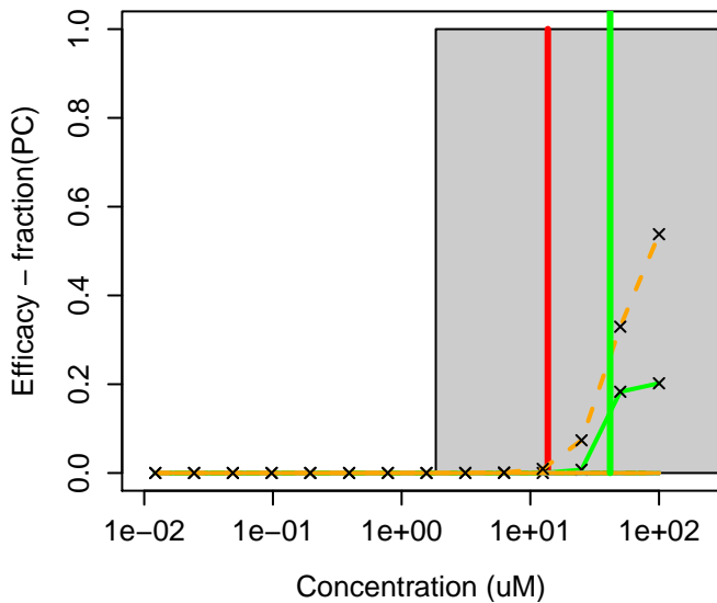
1330-78-5 : Tricresyl phosphate
