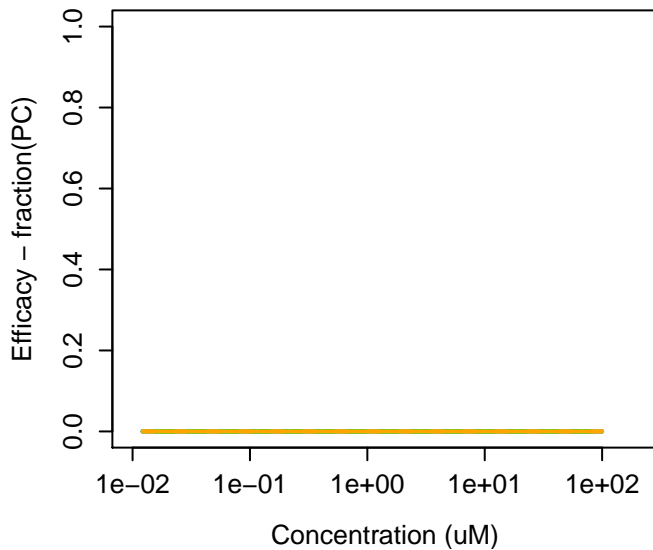
104-67-6 : 5-Heptyldihydro-2(3H)-furanone
