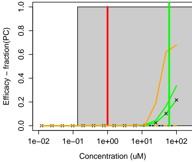
81-90-3 : Phenolphthalin
