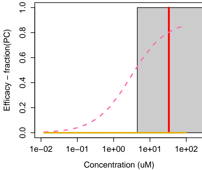
102-06-7 : 1,3-Diphenylguanidine
