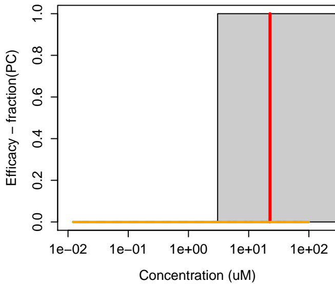
122-78-1 : Phenylacetaldehyde
