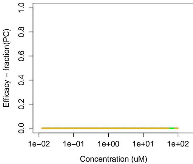
131-11-3 : Dimethyl phthalate
