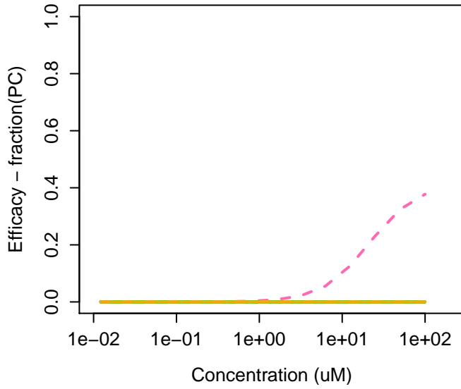
824-39-5 : Sodium 2-nitrophenolate
