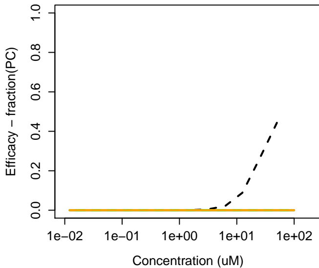
10025-74-8 : Dysprosium(III) chloride
