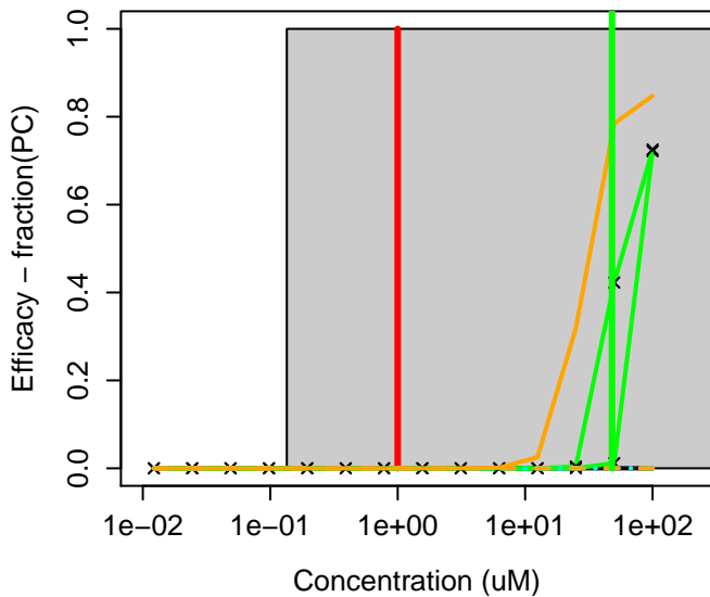
18979-55-0 : 4-(Hexyloxy)phenol
