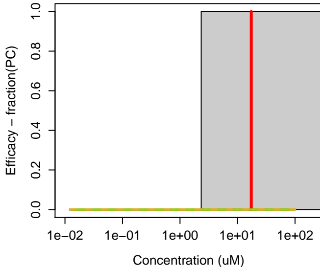
2244-21-5 : Potassium dichloroisocyanurate
