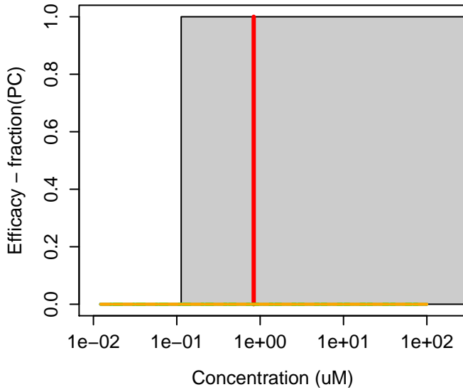
69806-40-2 : Haloxyfop-methyl
