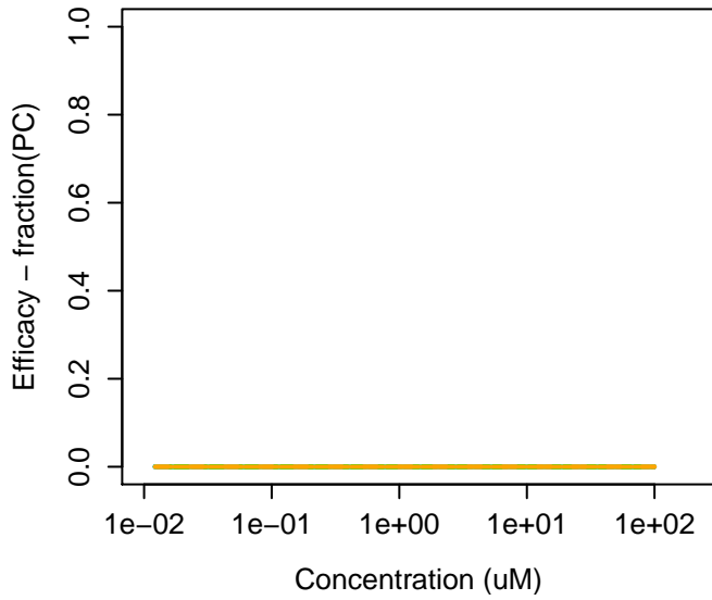
1861-32-1 : Chlorthal-dimethyl
