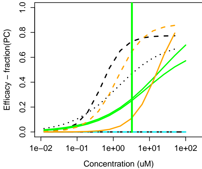
90-43-7 : 2-Phenylphenol
