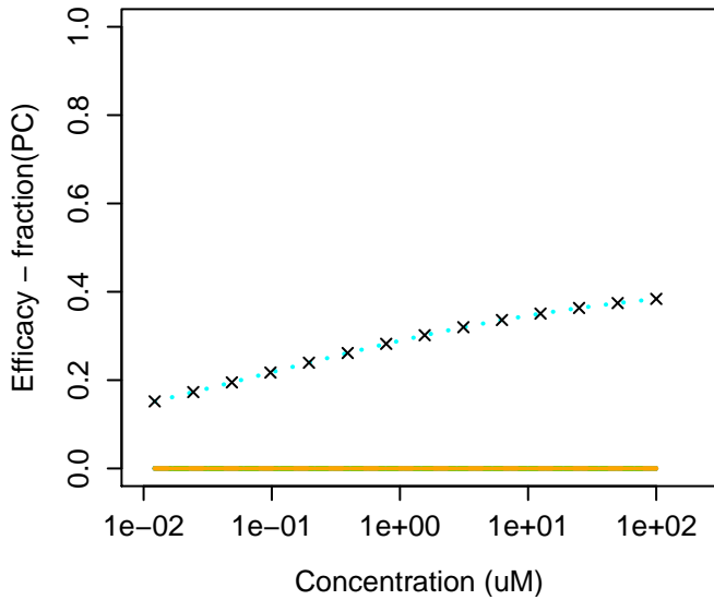
2687-96-9 : 1-Dodecyl-2-pyrrolidinone
