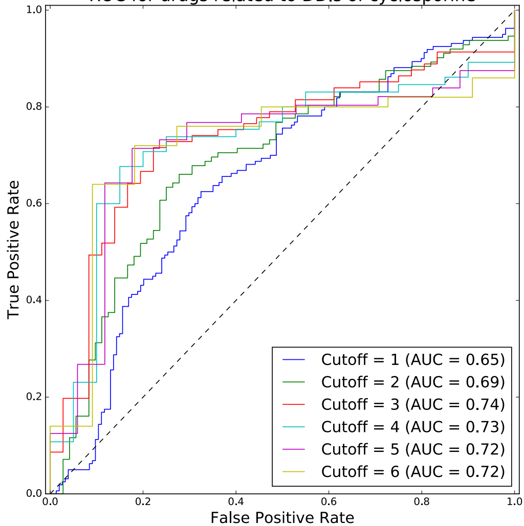
ROC for drugs related to DDIs of cyclosporine
