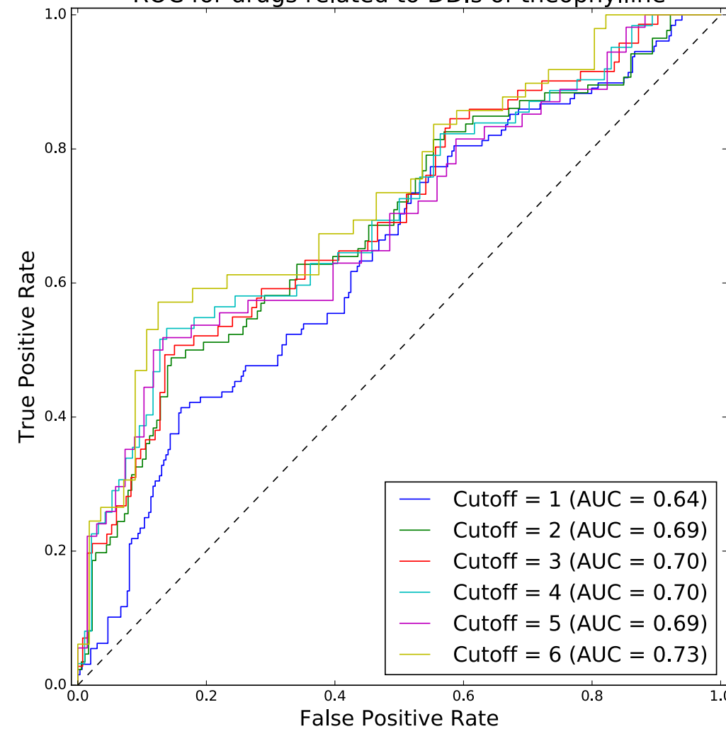
ROC for drugs related to DDIs of theophylline
