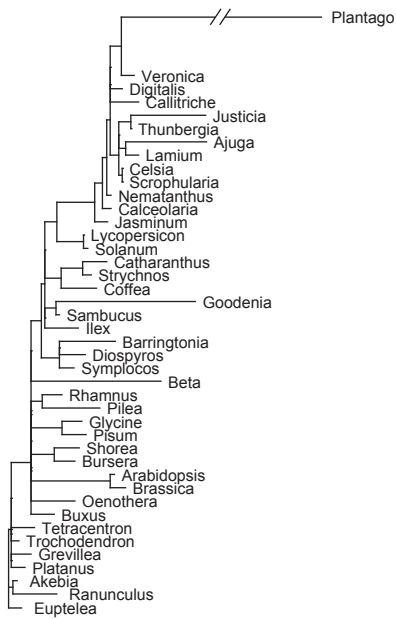
mt atp1 - d_S
