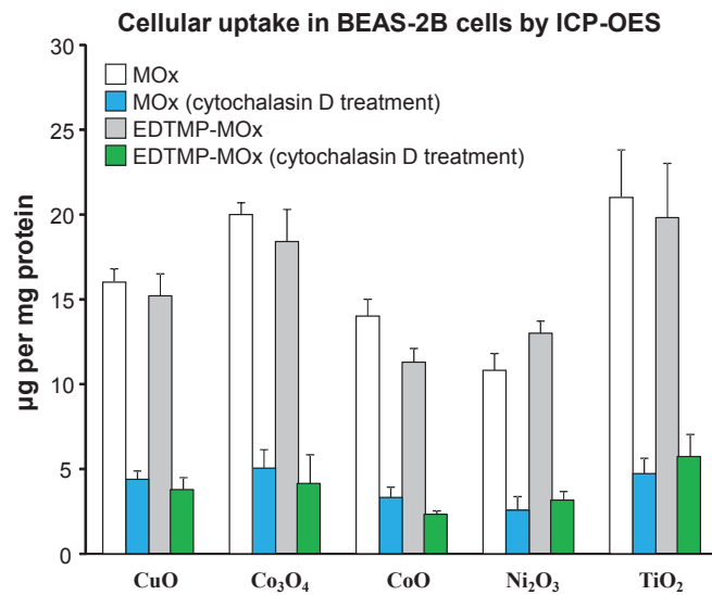
Figure S6. Influence of EDTMP coating to the cellular uptake mechanism of MOx. BEAS-2B cells pretreated with 5 µg/mL cytochalasin D for 3 h were incubated with 50 µg/mL nanoparticles for an additional 6 h. The cellular uptake levels of MOx were determined by ICP-OES.
