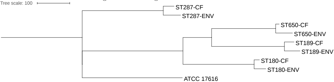
S1 Fig. Parsimony tree showing the relatedness of the genomes in terms of gene content. Scale bar represents number of changes of state required in each character. The tree was rooted on the branch with the largest branch length.
