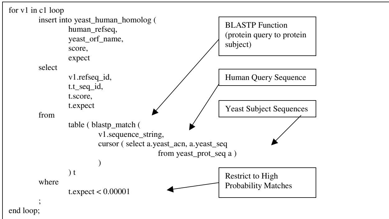
Figure 1. The PL/SQL Script for Performing the Iterative BLAST Query.
