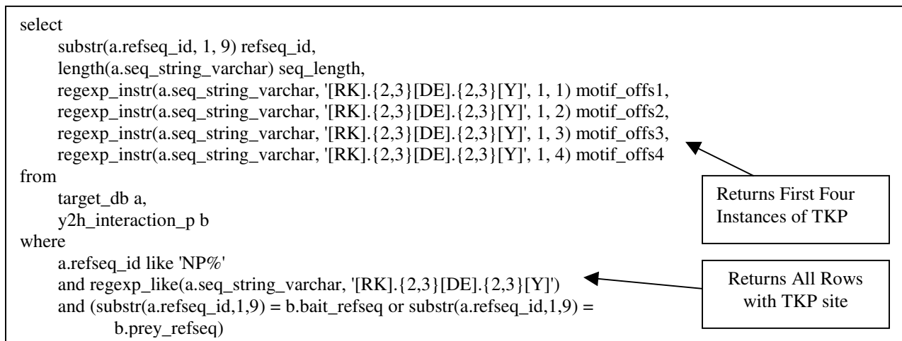
Figure 2. The SQL Statement for Identifying the Location of the First Four TKP Sites in a Protein Database.
