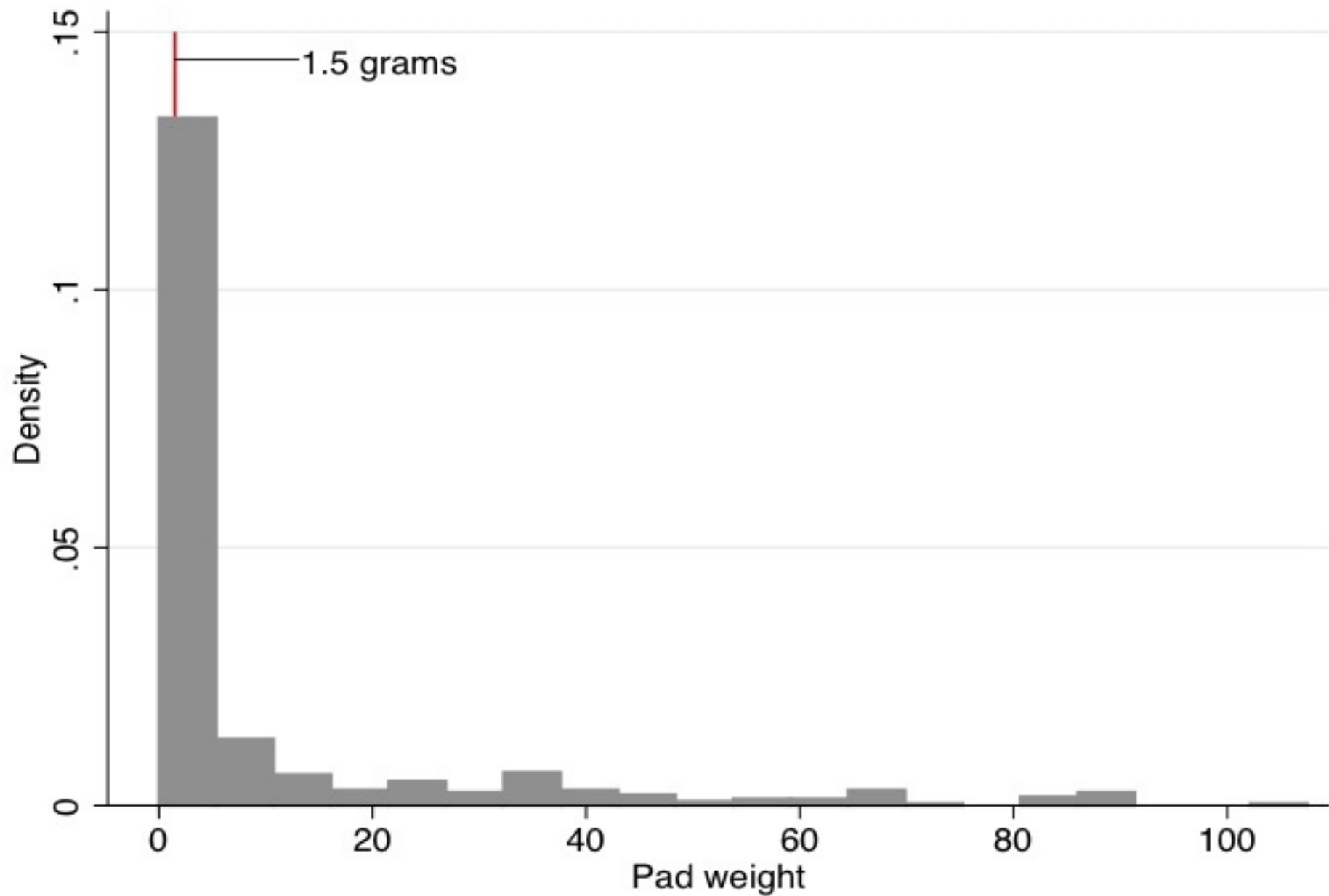
Figure S1: Distribution of the weights of post-operative 1-hour pad testing
