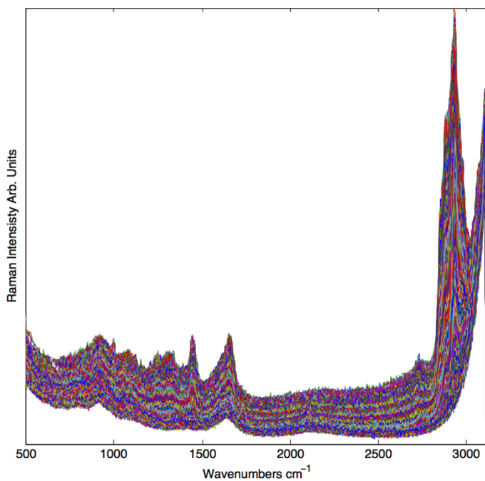
Figure S1: Example of Raw data before Extended Multiplicative Scater Correction and Spectral Interference Subtraction (EMSC-SIS), Correction spectra.
