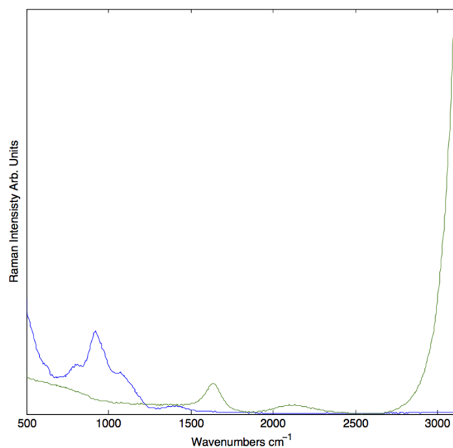
Figure S2: Spectra of water (green) and glass (blue) used for correction of backgrounds.
