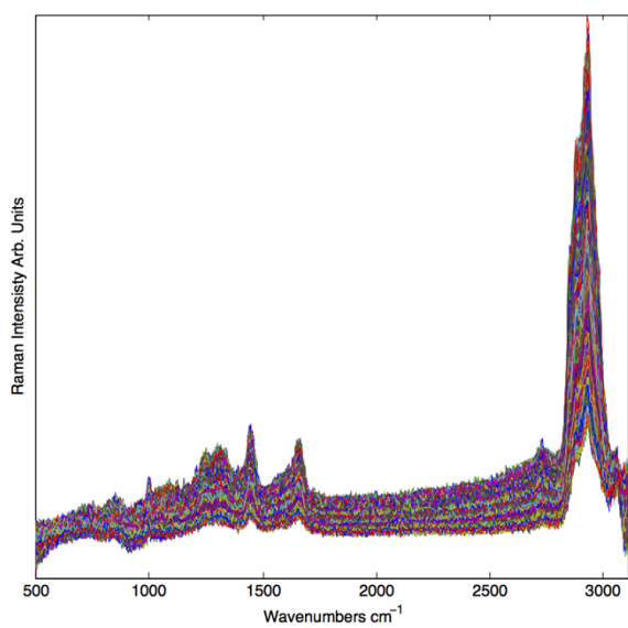
Figure S3: Dataset after correction using EMSC-SIS.
