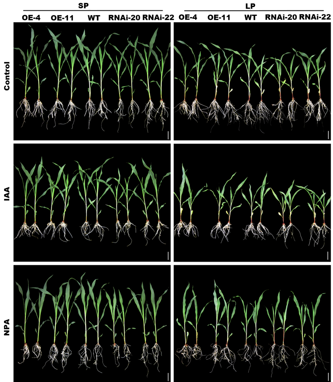
S3 Figure. Representative seedlings grown for 15d under SP (left) or LP (right) solution with or without IAA or NPA. Bar=5 cm.
