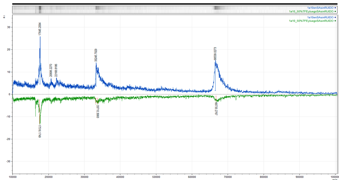
Figure S1. Molecular mass determination by MALDI TOF/TOF of the 66 kDa polypeptide formed after treatment of the Vip3Aa protoxin with trypsin (24:100 trypsin:Vip3A, w:w) for 3 days.
