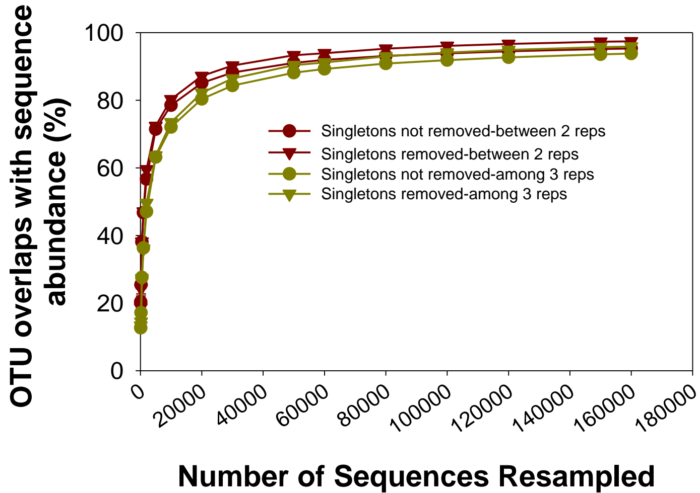
S3 Fig. Sequence abundance weighted OTU Overlaps generated with using Uclust between/among technical replicates at different sequencing depth. At a sequencing depth of about 30,000 reads, overlaps of both two and three replicates were reaching a plateau no matter singletons were removed or not.
