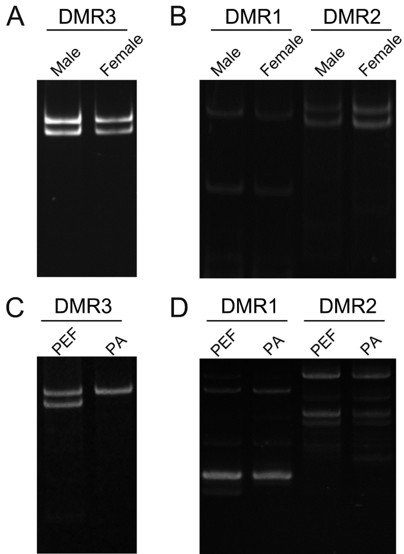
Figure S1 - Methylation pattern of H19 DMD and IGF2 DMRs. For COBRA analysis, the PCR products of H19 DMD and IGF2 DMRs were digested with the restriction enzyme Taq I in male and female eye (A and B), and porcine embryonic fibroblast (PEF) and parthenogenetic (PA) cells (C and D), respectively.
