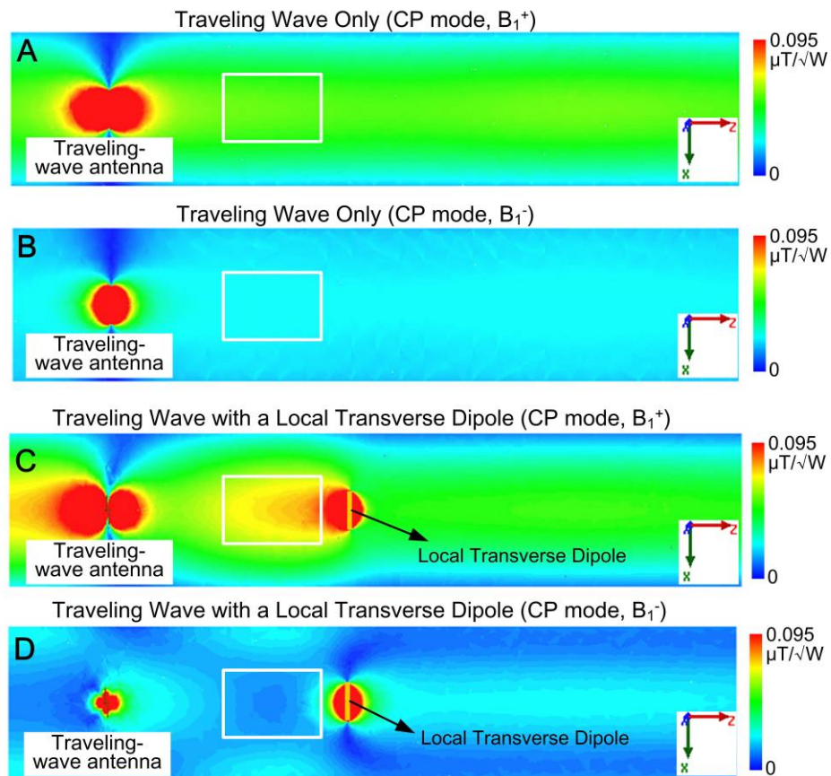
Figure S1 Simulated B_{1+} and B_{1-} maps in CP mode without local coils ( A and B ) and with a local transverse dipole ( C and D ). The ratio between B_{1+} and B_{1-} in CP mode increases locally (white box) when loaded with a local transverse dipole, which might also contribute to transmit efficiency improvement.
