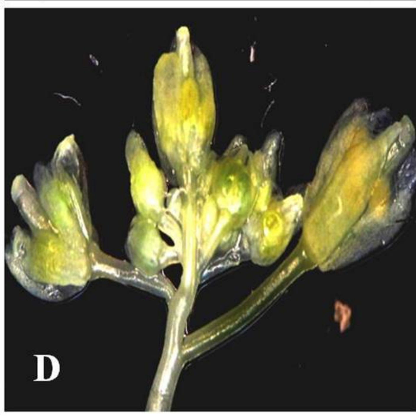
Supplemental Figure S8. GUS expression in transgenic Arabidopsis plants carrying pAtHEMN1::uidA construct. GUS expression was not found in seedlings (A), roots (B), or internodes (C) but was observed in flower buds (D).
