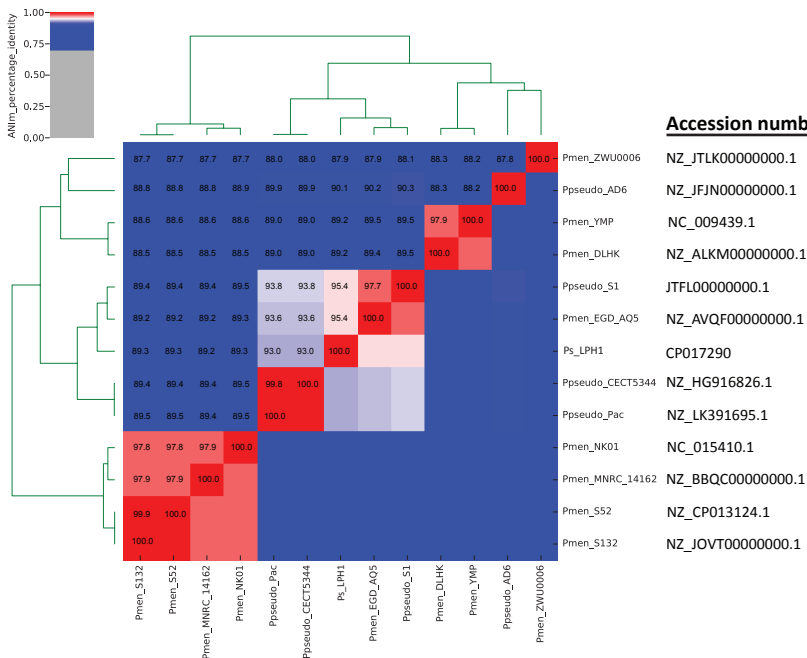
Fig. S1. Pseudomonas species comparative genomics. Average Nucleotide Identity (ANI) analysis and clustering were performed using PyANI (Richter M & Rossello-Mora R, PNAS 2009, 106 (45): 19126-31, and https://github.com/widowquinn/pyani ) of Pseudomonas isolate LPH1 and twelve closely related Pseudomonas species. Ppseudo, Pseudomonas pseudoalcaligenes ; Ps_LPH1, Pseudomonas isolate described in this paper; Pmen, Pseudomonas mendocina .
