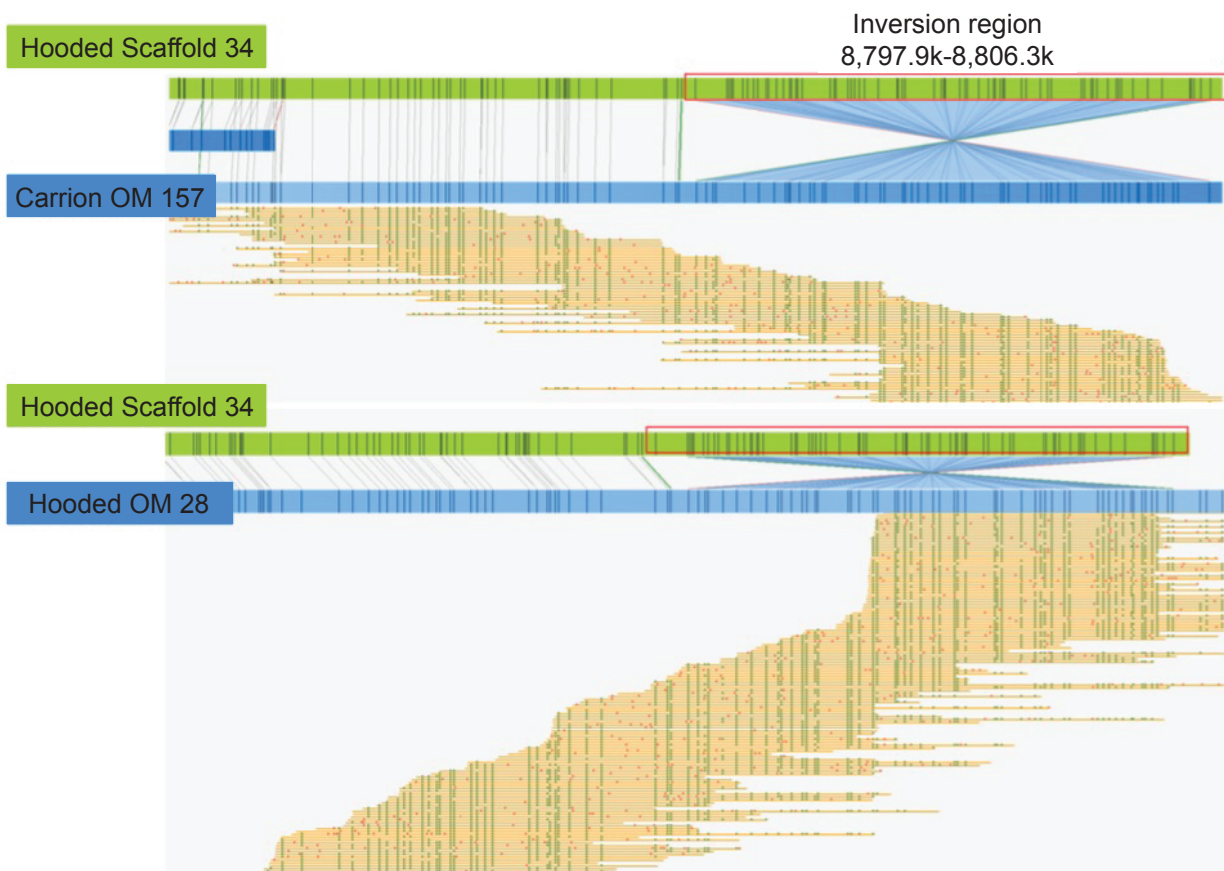
Supplemental Figure S1: Example for an artificial inversion in the SR assembly identified by OM alignment.
