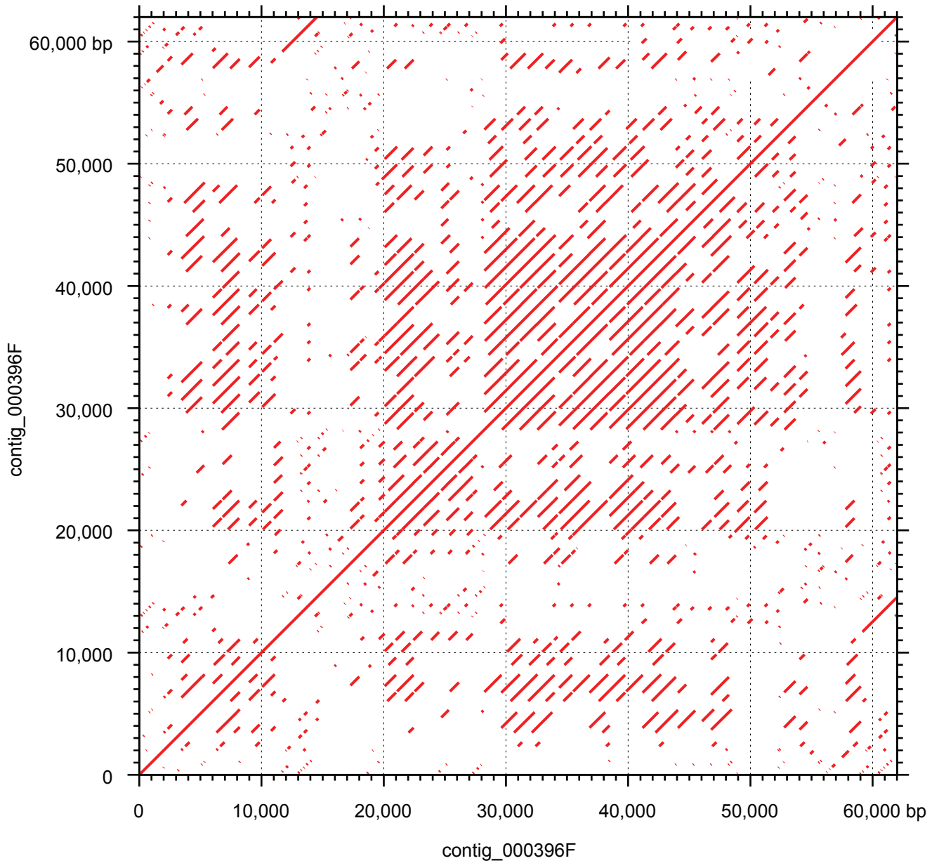
Supplemental Figure S4: Sequence similarity plot of a self-alignment of an LR contig (contig_000396F) entirely consisting of tandemly repeated crowSat1 subunits.
