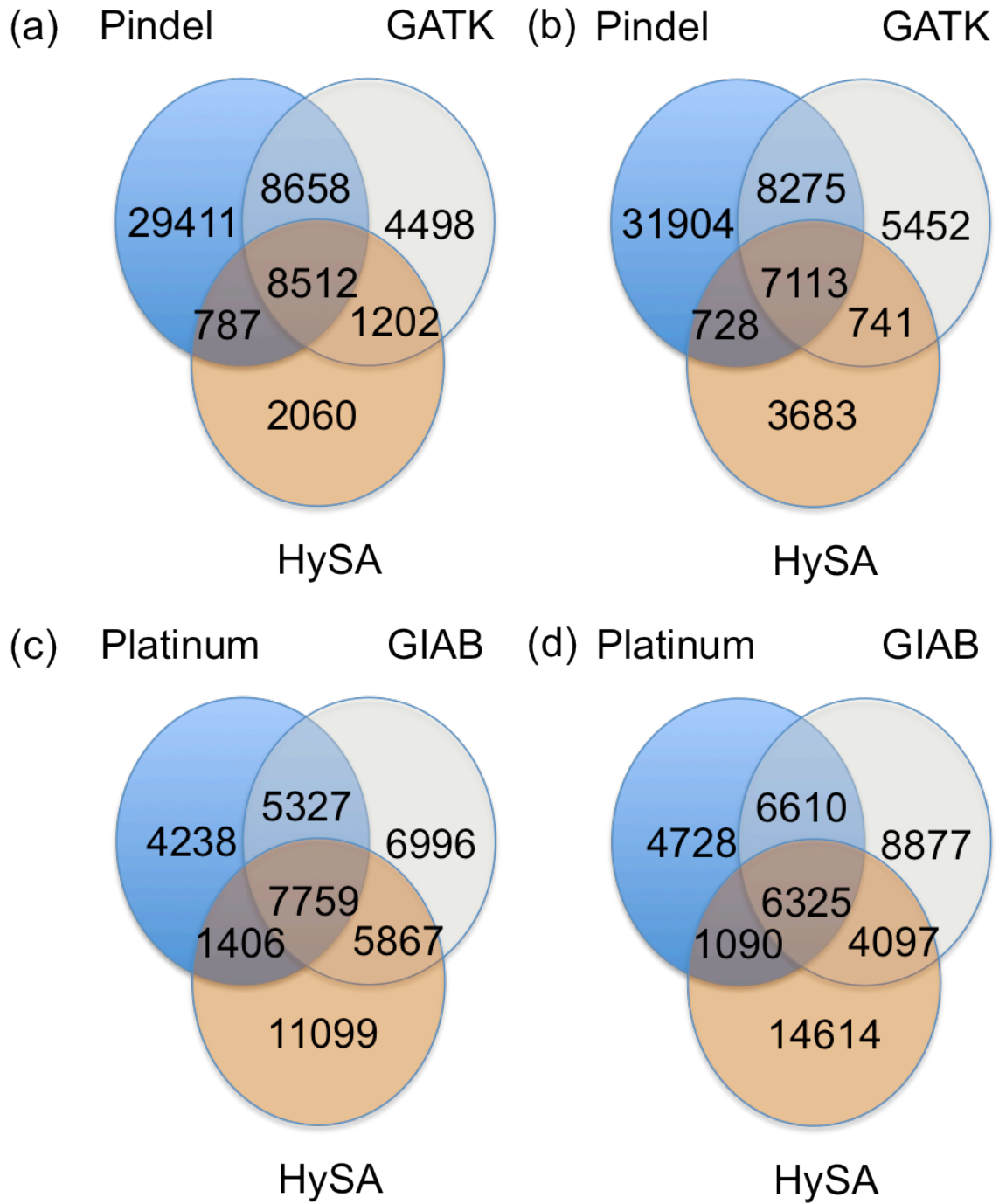
Supplemental Fig. 5 Venn diagram of small insertion calls of CHM1 with (a) 30bp and (b) 10bp padding; and NA12878 with (c) 30bp and (d) 10bp padding.
