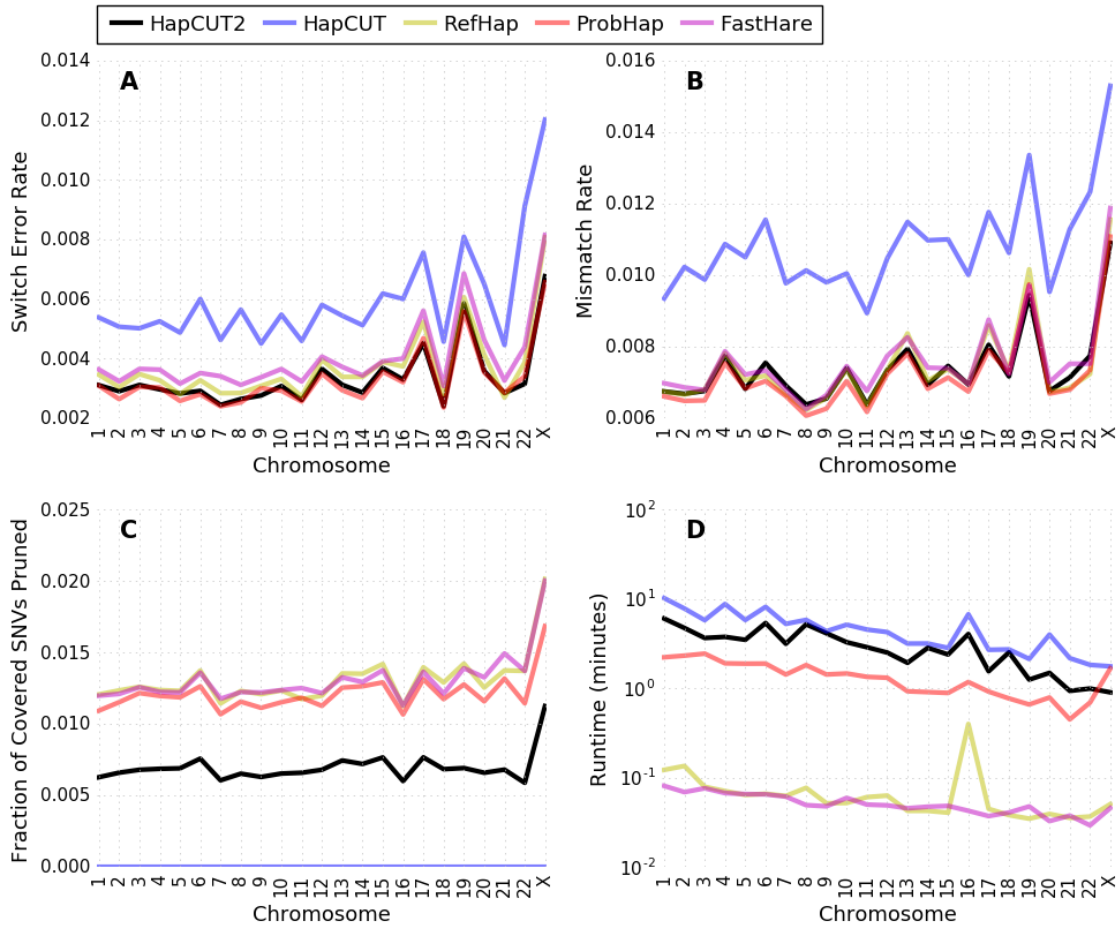
Figure S2: Comparison of the performance of HapCUT2 with other tools on NA12878 fosmid data across all chromosomes: (A) Switch error rate, (B) Mismatch rate, (C) Fraction of covered variants pruned, and (D) Runtime in CPU-minutes. Switch and mismatch errors were calculated using the set of phased variants specific to each tool.
