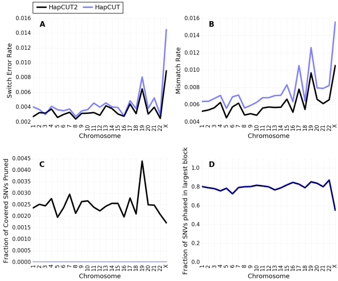
Figure S6: Comparison of HapCUT2 to HapCUT on 90 \times coverage MboI Hi-C data. (A) Switch error rate (B) Mismatch rate (C) Fraction of covered variants pruned (D) Fraction of variants phased in largest block. Switch and mismatch errors reported here are for all variants phased by a given tool, so the fraction of variants pruned is also reported.
