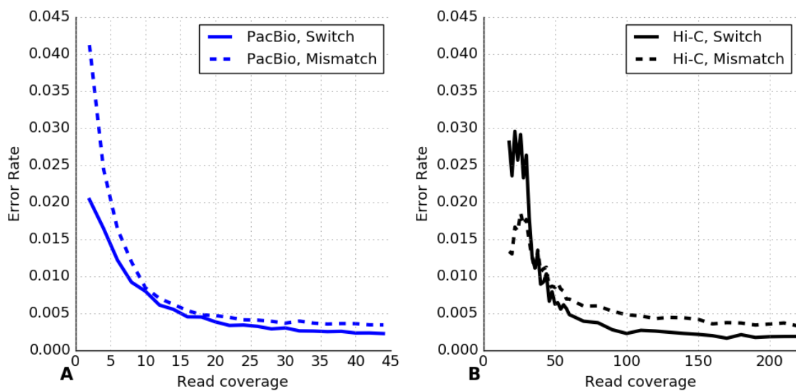
Figure S7: Haplotype accuracy (switch and mismatch error rates) for the NA12878 genome as a function of sequence coverage for (A) PacBio SMRT data and (B) Hi-C (MboI enzyme) data.
