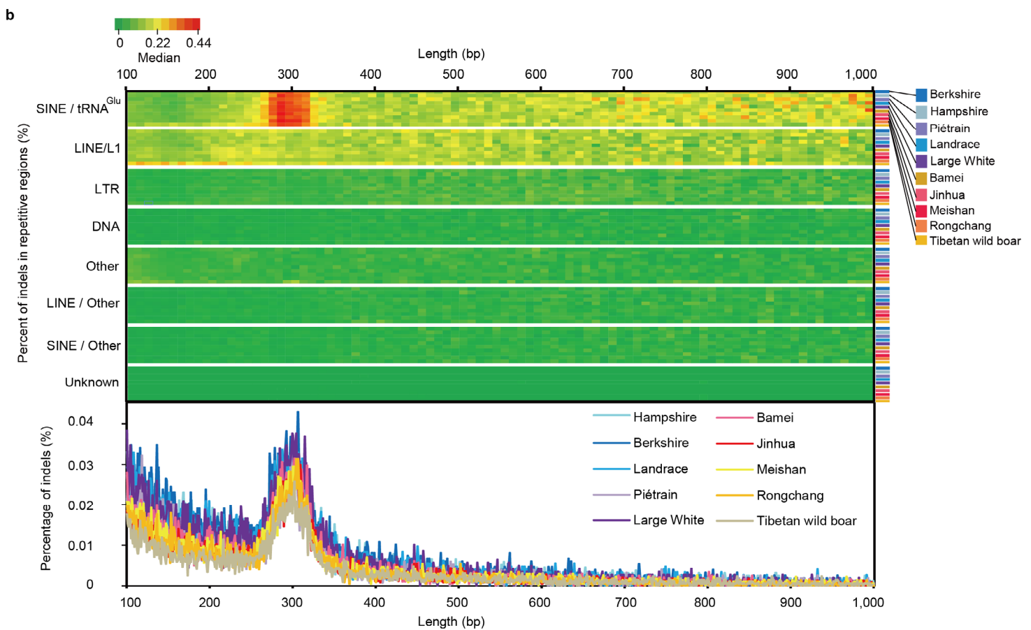
Supplemental Fig. S17. Length distribution of indels. (a) Overall distribution of the lengths of indels. (b) Distribution of indel between 100 bp and 1 kb in length. Peak at ~300 bp (bottom panels) is due to the enrichment of indels of tRNA Glu -derived short interspersed element (SINE/tRNA Glu ) (top panels).
