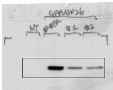
Anti-GFP
