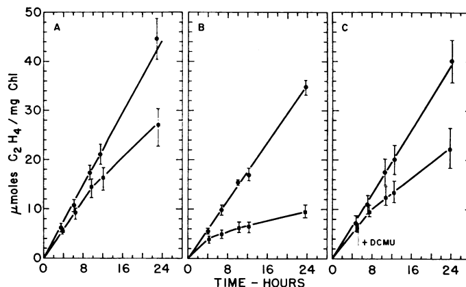
FIG. 2. Effect of DCMU and light or dark pretreatment on acetylene reduction by the symbiotic association under microaerophilic conditions. A: Fronds maintained under light (750 ft-c), aerobic conditions 12 hr prior to incubation under microaerophilic conditions. ●: control; ■: DCMU-treated; 12 \mu M added at time zero. B: Fronds maintained in darkness under aerobic conditions for 12 hr prior to incubation, otherwise as for A. C: Same as B except fronds left in light 5 hr before adding DCMU.
