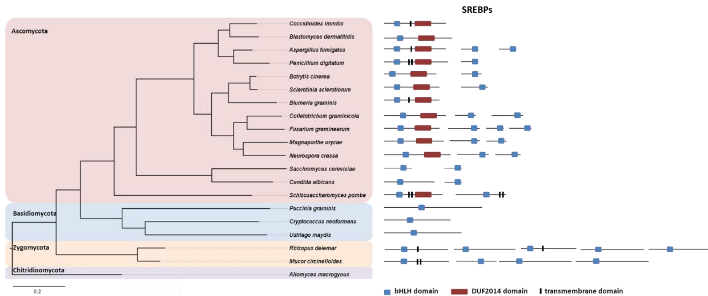
S2 Fig. Evolution of SREBPs in fungi. Phylogenetic tree was constructed by concatenating 27 conserved ribosome proteins using MEGA6. The number and gene structure of SREBPs in fungi were annotated. Domain information was obtained from the pfam database.
