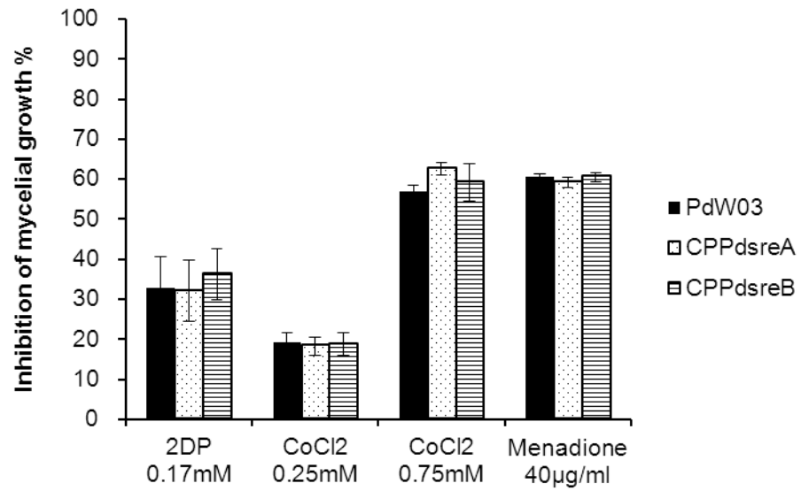
S3 Fig. Sensitivity of the wild-type PdW03 and the complementation strains to 2DP, CoCl 2 and menadione.
