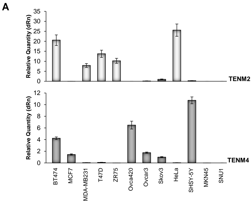
S1 Fig. Additional RT-PCR Data of Ten-1 and Ten-2 Transcripts.
