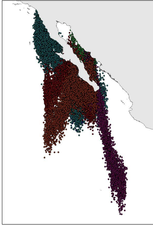
Figure S2 Resampled locations (point density data) along previously reported tag-specific longitudinal
